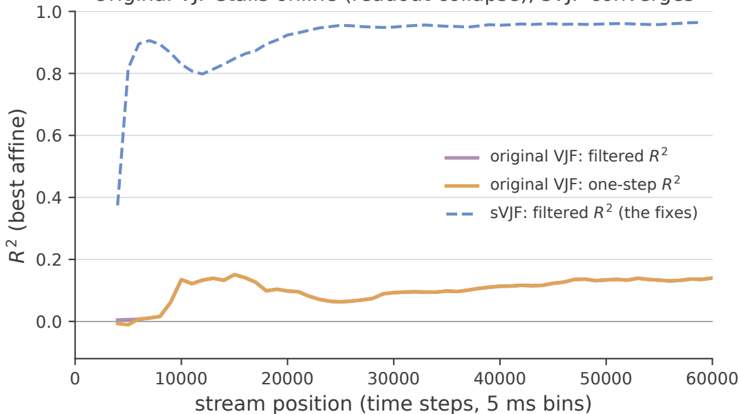
Original VJF stalls online (readout collapse); sVJF converges
