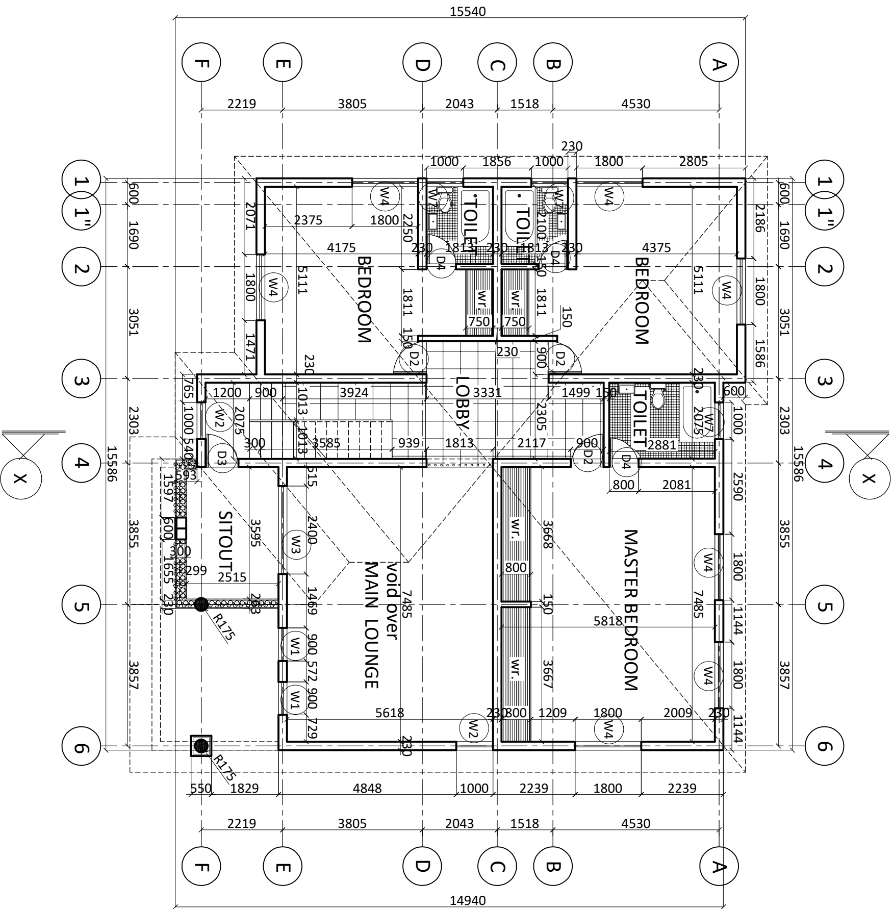
UPPER FLOOR PLAN (scale ..... 1 : 100)
