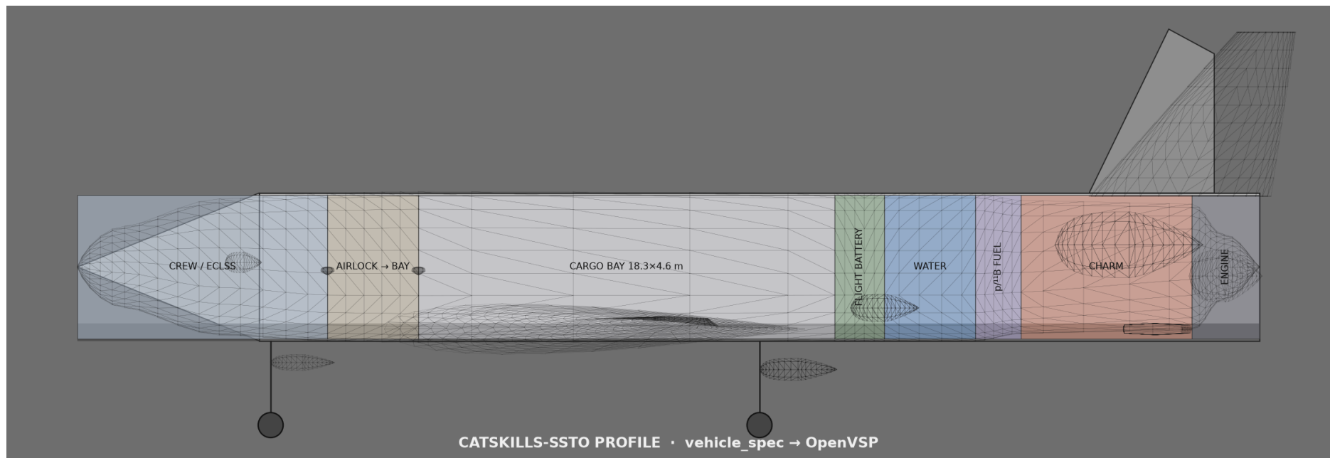
Figure 4 Vehicle profile view.
