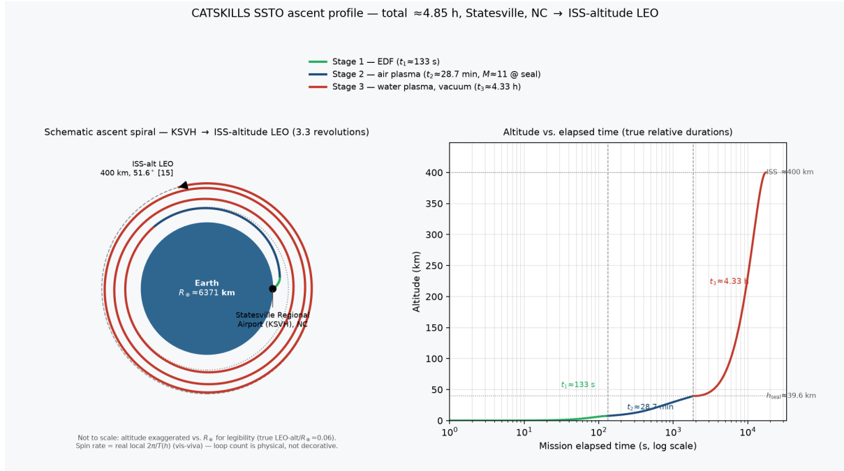
Figure 17 Schematic ascent profile from Statesville Regional Airport (KSVH), NC to ISS-altitude LEO ( \approx 400 km, 51.6^\circ [15]): spiral view (left, altitude exaggerated, colored by stage) and altitude vs. mission elapsed time on a log time axis (right, true relative stage durations). Generated by emit_orbital_ascent_diagram.py .
