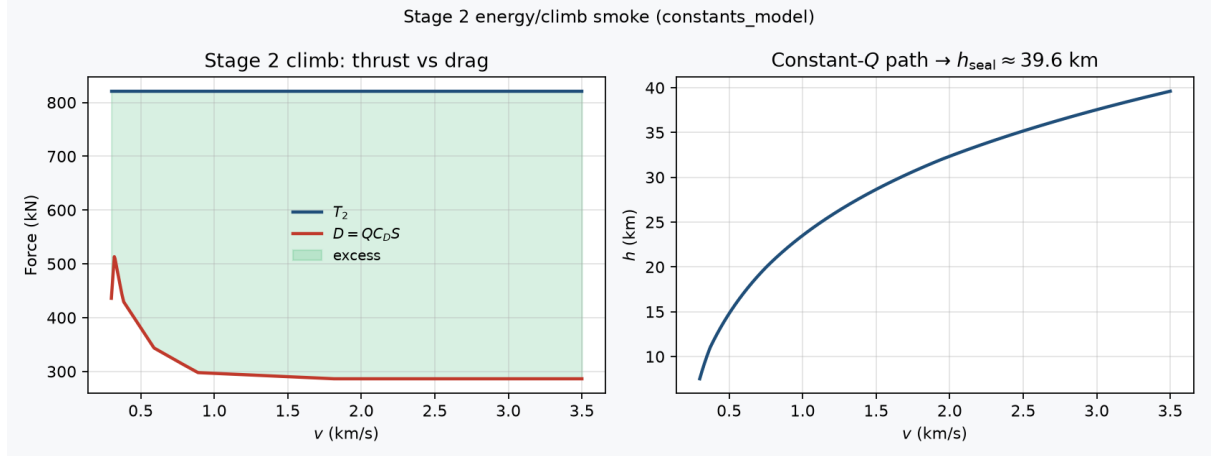
Figure 13 Stage 2 climb smoke: constant- Q path with T_2 vs D = QC_D S (left) and h(v) to seal (right).
