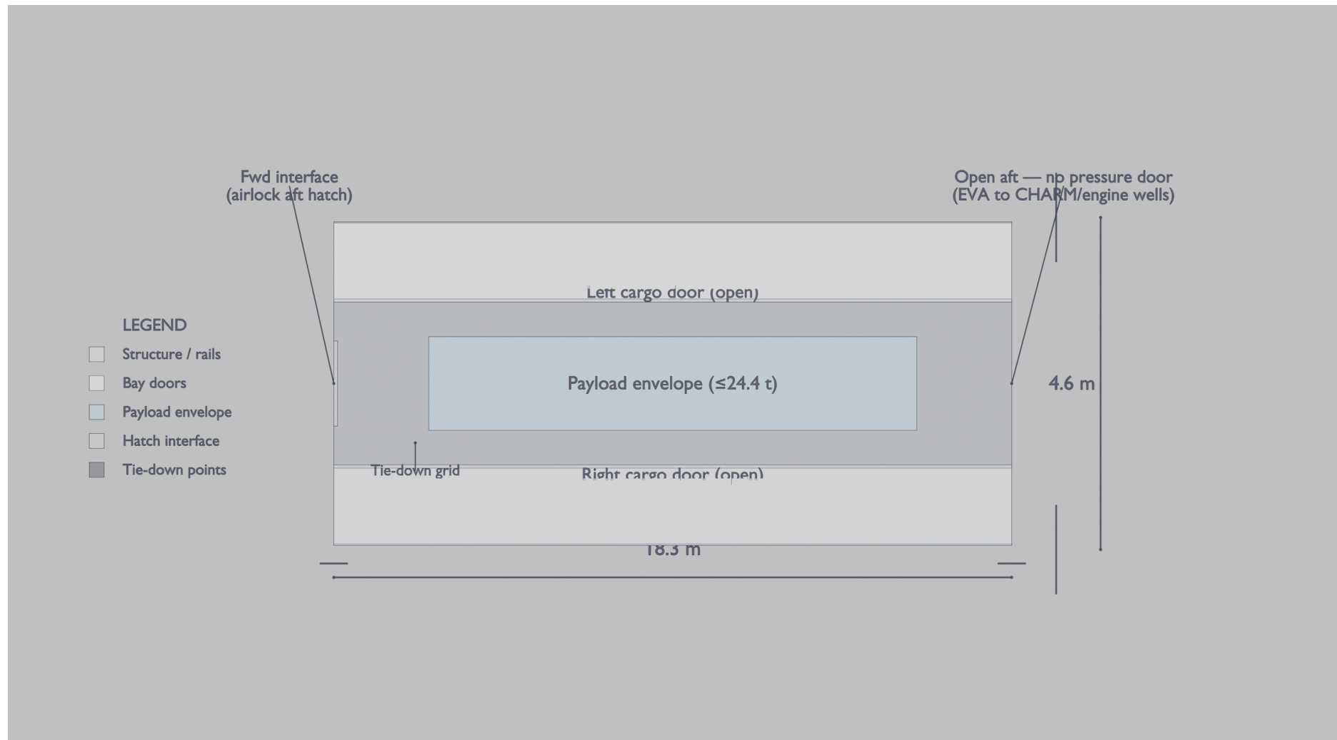
Figure 5 Cargo skid, Blender top-down cutaway from assembly.json with bay doors open.
