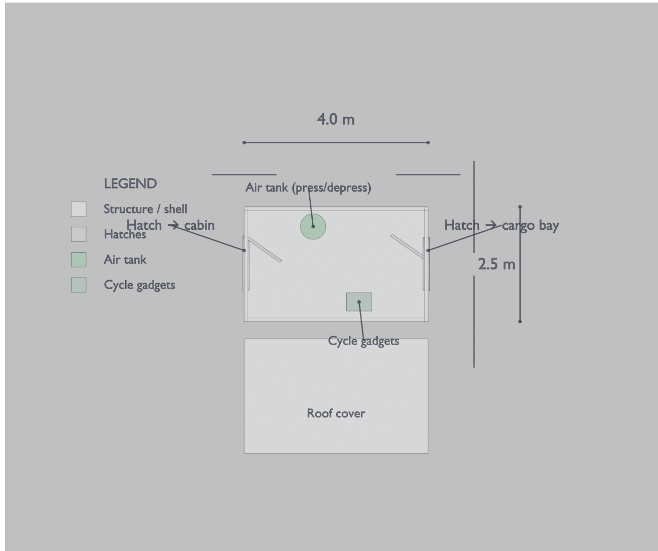
Figure 4 Airlock, Blender top-down cutaway from assembly.json.
