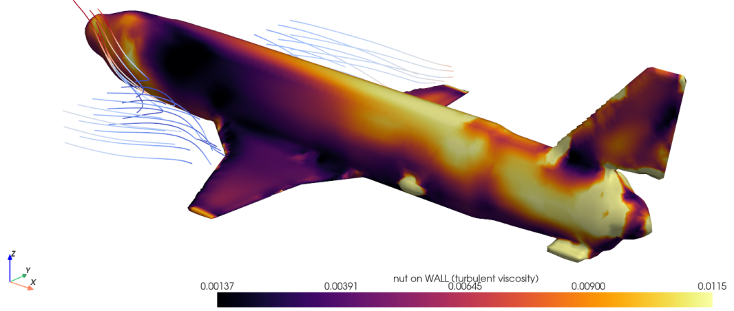
Figure 13 Stage 1 turbulent flow: OpenFOAM Spalart–Allmaras RANS ( \sim M = 0.3 , \alpha = 4^\circ ), full airframe. Wall coloured by eddy viscosity \nu_t ; streamlines over the forward fuselage and wing root.
