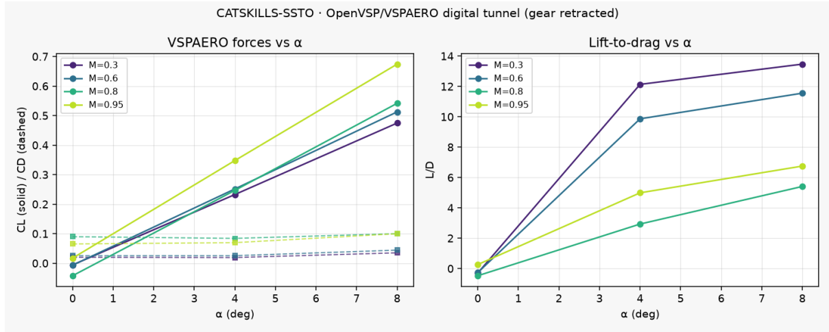
Figure 11 Stage 1 VSPAERO polar (Mach \times\alpha digital tunnel on catskills_ssto.vsp3 ).
