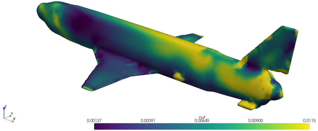
Figure 12 Stage 1 snappyHexMesh wall on the OpenVSP exterior (full airframe in frame; unbroken tube OML — bay doors live on the cargo-skid drop-in, not as roof wings). Colour = wall eddy viscosity \nu_t from the Stage 1 RANS dump.
