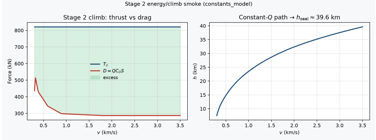
Figure 15 Stage 2 climb smoke: constant- Q path with T_2 vs D = QC_D S (left) and h(v) to seal (right).
