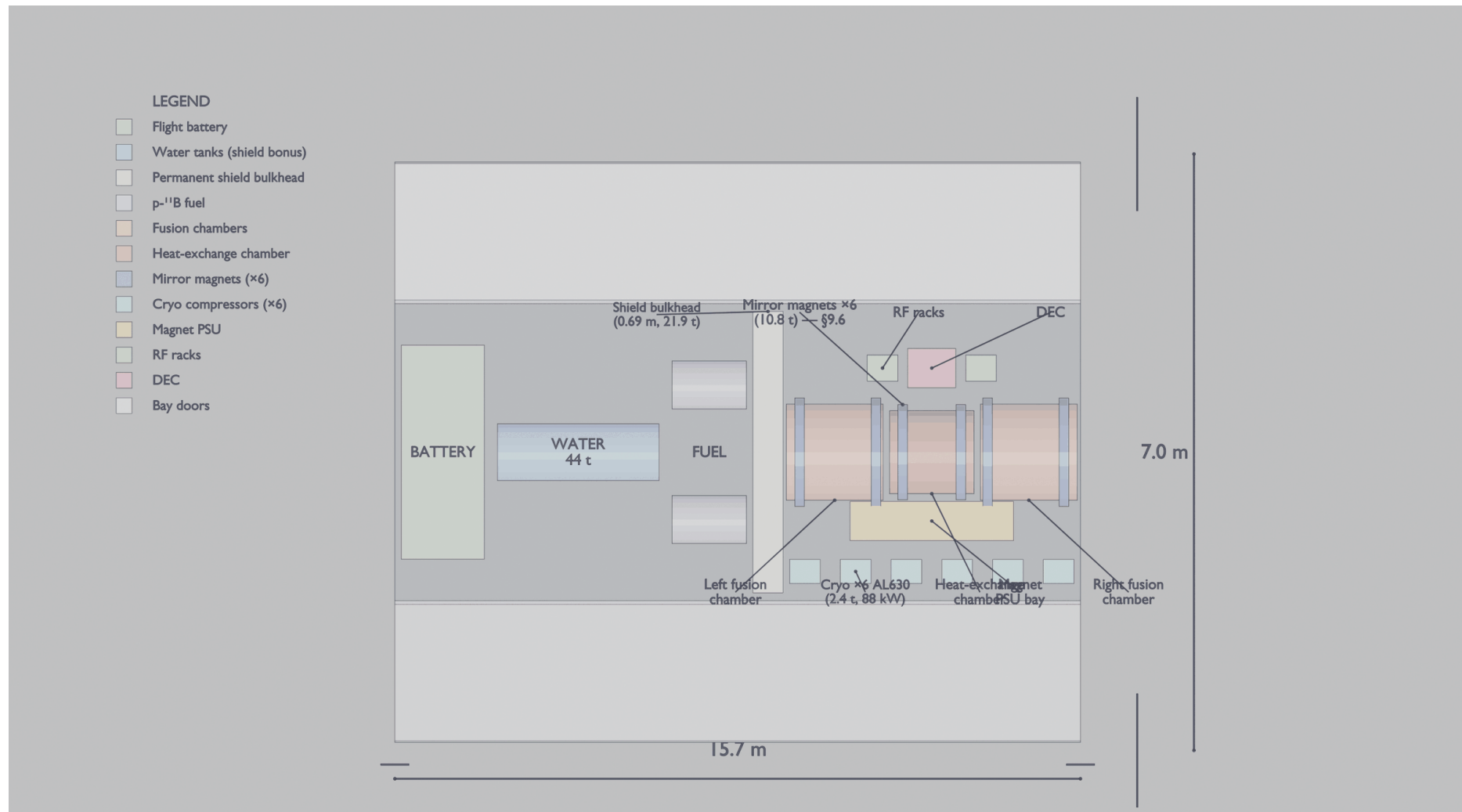
Figure 8 Fusion plant skid, Blender top-down cutaway from assembly.json: flight battery, relocated water tanks (radiation-shield buffer, $9.9), p-11B fuel, permanent shield bulkhead, chamber string, 6 mirror magnets, 6-unit cryo compressor bay, magnet PSU, RF, and DEC.
