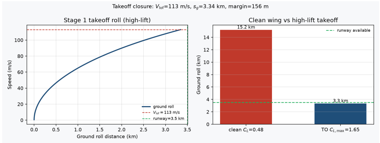
Figure 14 Stage 1 takeoff closure: ground-roll speed vs distance (left); clean-wing vs high-lift runway demand (right).
