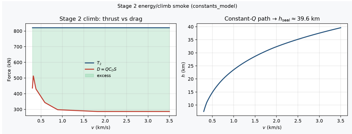
Figure 15 Stage 2 climb smoke: constant- Q path with T_2 vs D = QC_D S (left) and h(v) to seal (right).
