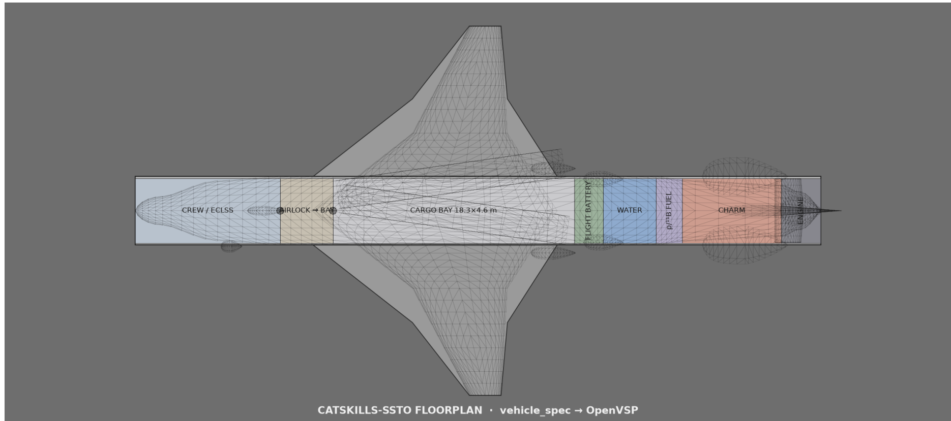
Figure 1 Vehicle floor plan.
