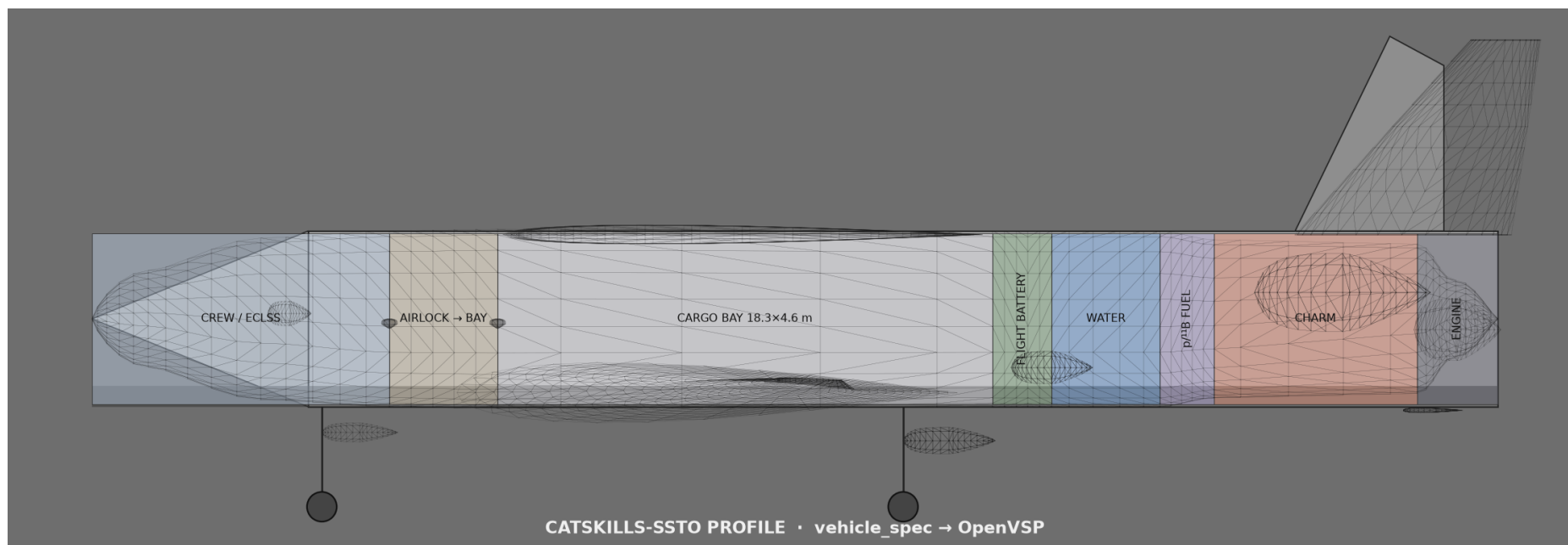
Figure 2 Vehicle profile view.
