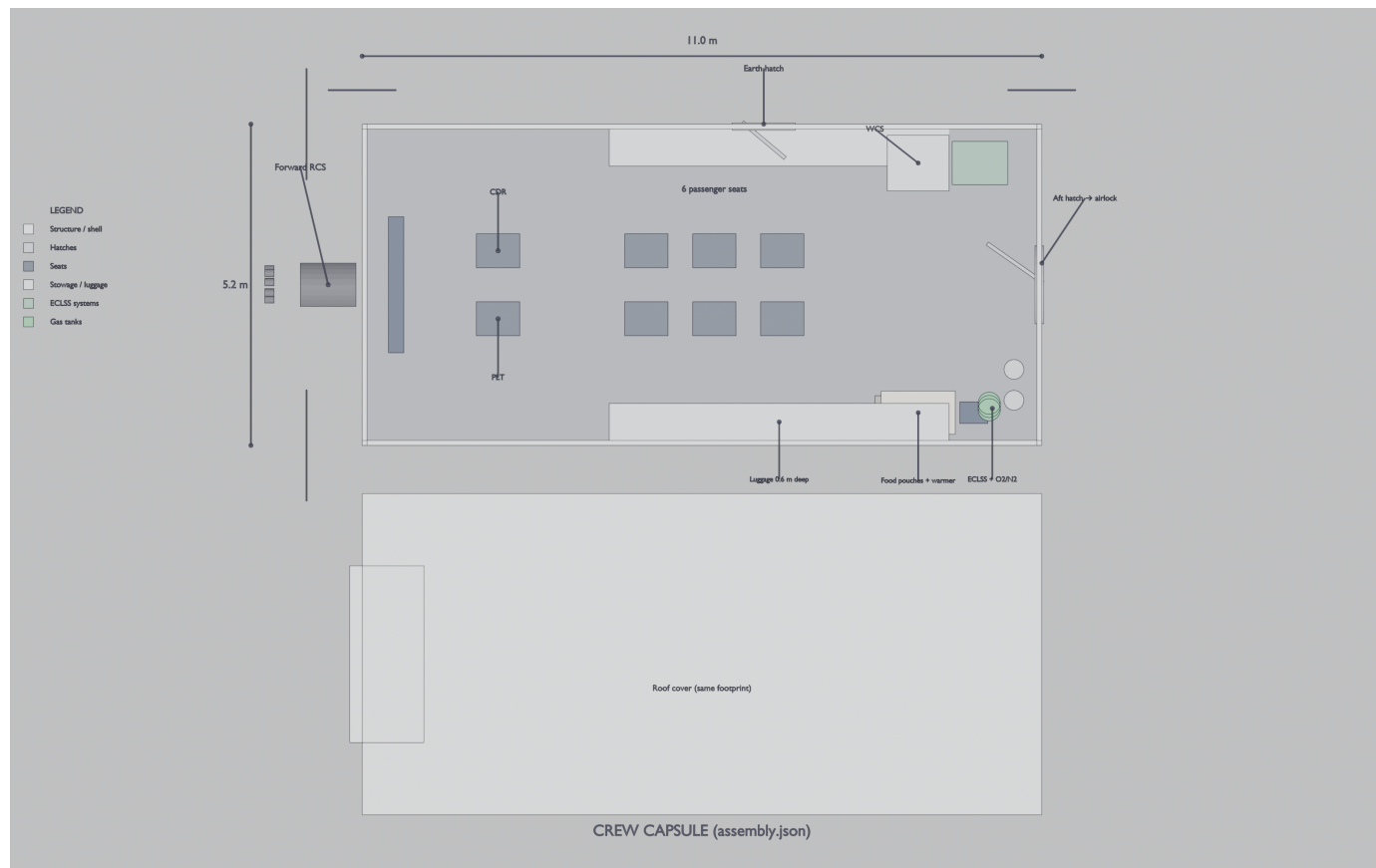
Figure 3 Crew capsule, Blender top-down cutaway from assembly.json.
