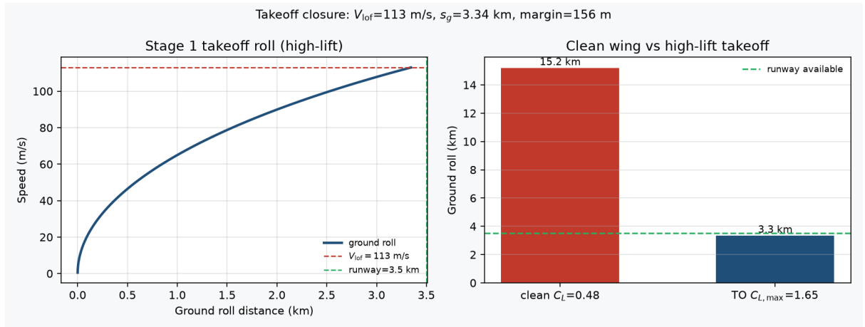
Figure 12 Stage 1 takeoff closure: ground-roll speed vs distance (left); clean-wing vs high-lift runway demand (right).
