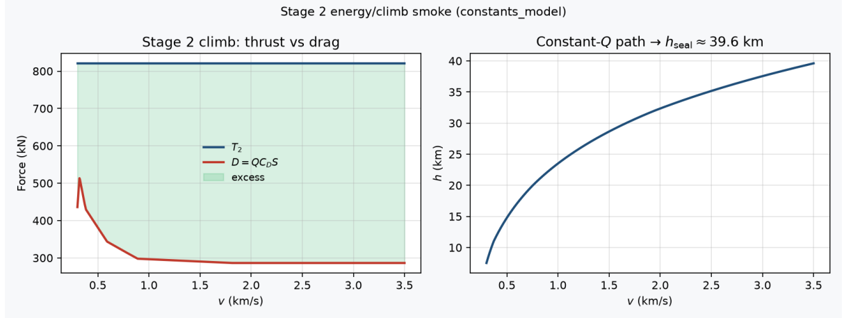
Figure 13 Stage 2 climb smoke: constant- Q path with T_2 vs D = QC_D S (left) and h(v) to seal (right).
