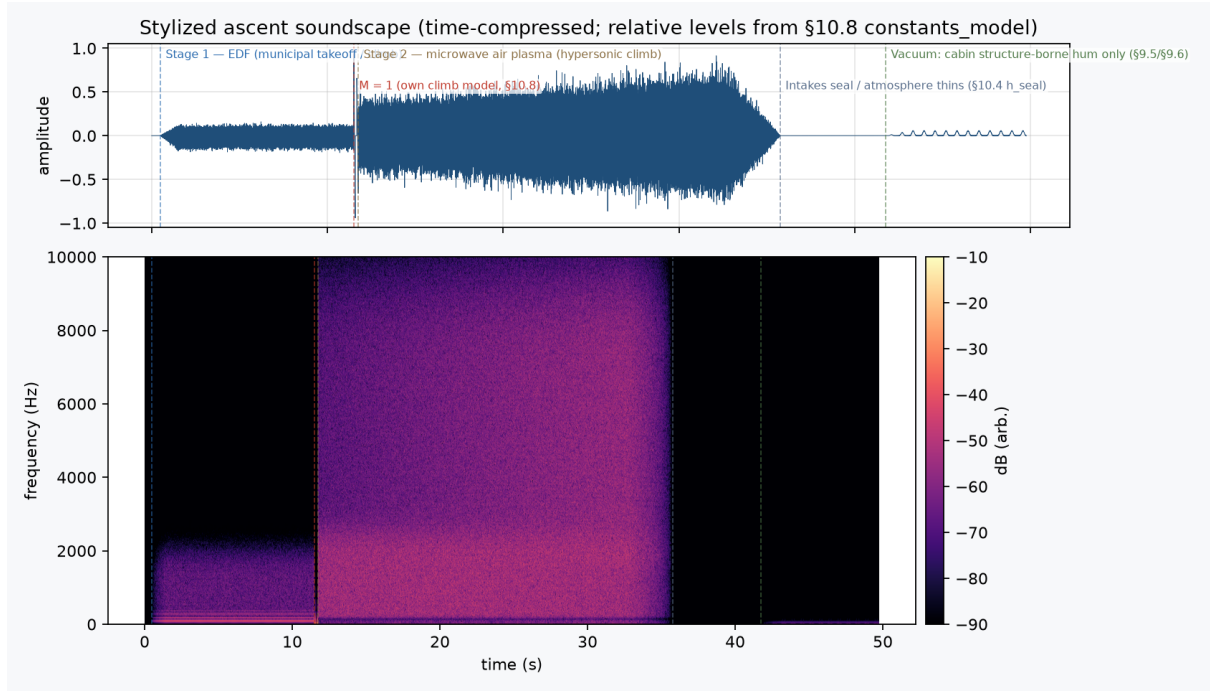
Figure 14 Ascent soundscape: waveform (top) and spectrogram (bottom) of the stylized audio signature — Stage 1 EDF, the modeled M = 1 crack, Stage 2 air-plasma roar, and the Stage-3 vacuum hum, in relative-loudness proportion from the table above.
