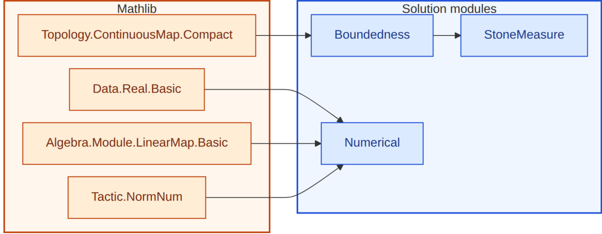
Figure 13: Lean module dependencies for the 21-720 solution. Amber box: Mathlib imports. Blue box: solution modules.
