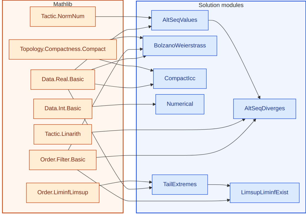
Figure 7: Lean module dependencies for the 21-355 solution. Amber box: Mathlib imports. Blue box: solution modules.
