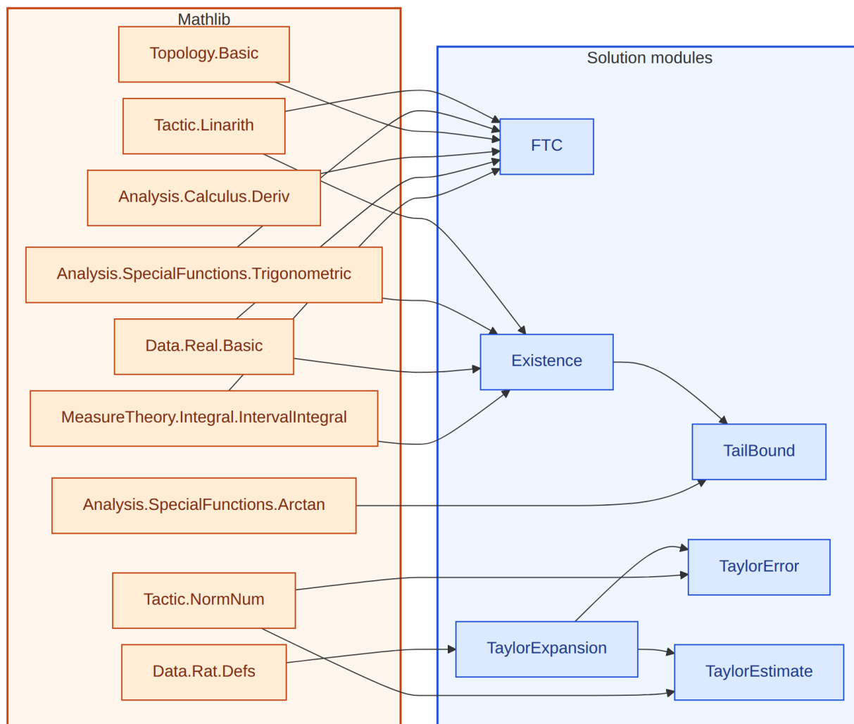
Figure 3: Lean module dependencies for the 21-120 / 21-122 solution. Amber box: Mathlib imports. Blue box: solution modules.
