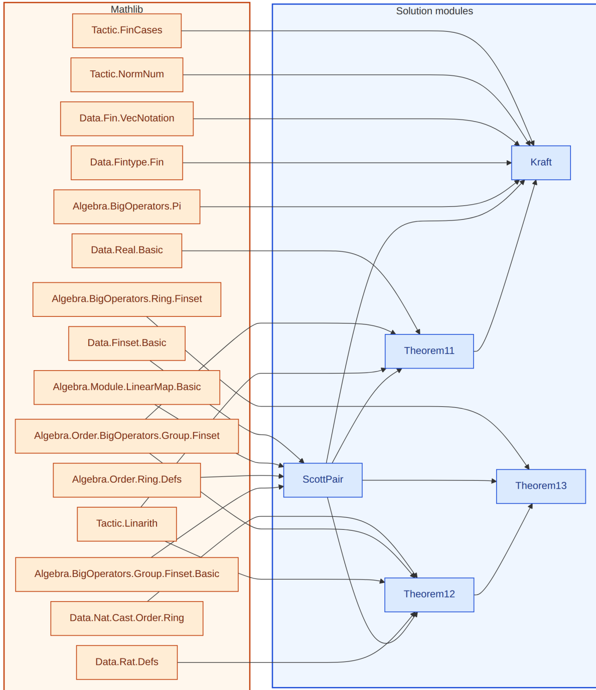
Figure 9: Lean module dependencies for the 21-321 solution. Amber box: Mathlib imports. Blue box: solution modules.
