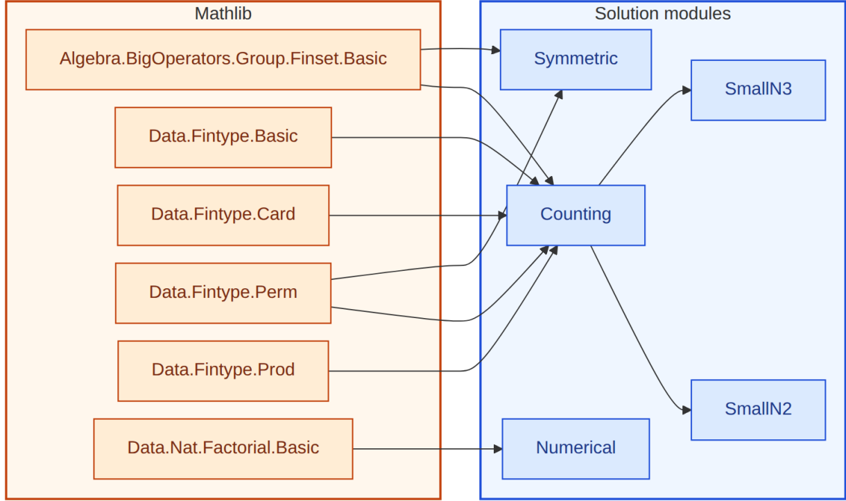
Figure 6: Lean module dependencies for the 21-228 solution. Amber box: Mathlib imports. Blue box: solution modules.
