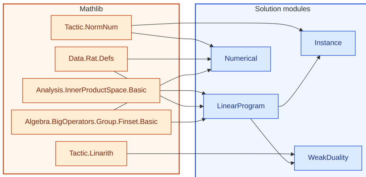
Figure 10: Lean module dependencies for the 21-292 solution. Amber box: Mathlib imports. Blue box: solution modules.
