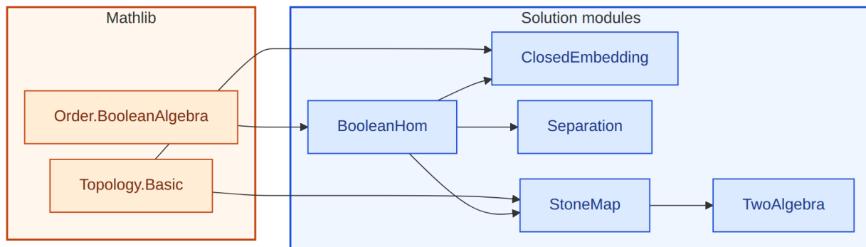
Figure 12: Lean module dependencies for the 21-651 solution. Amber box: Mathlib imports. Blue box: solution modules.
