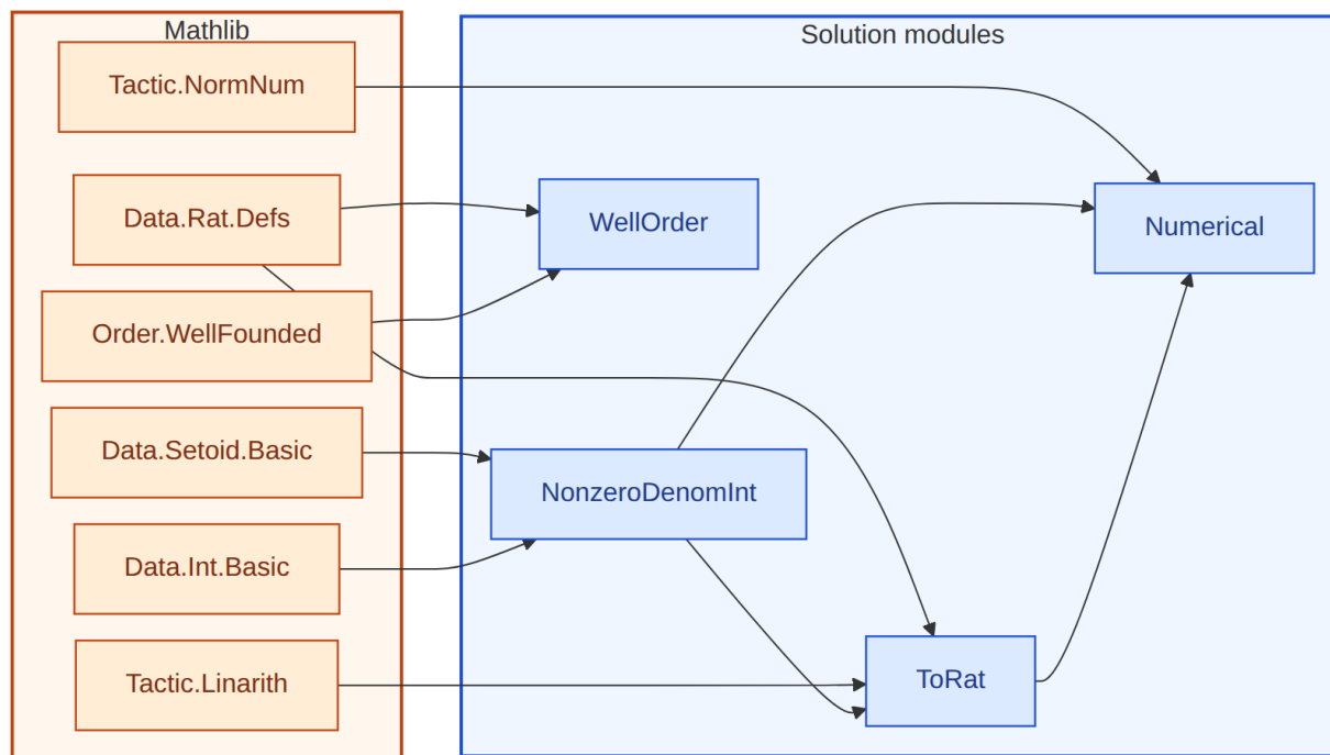
Figure 4: Lean module dependencies for the 21-127 solution. Amber box: Mathlib imports. Blue box: solution modules.
