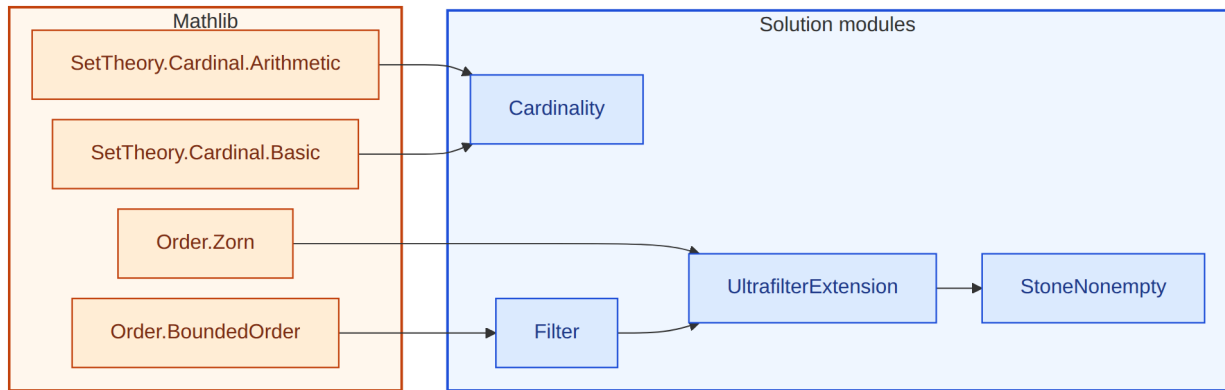
Figure 11: Lean module dependencies for the 21-329 solution. Amber box: Mathlib imports. Blue box: solution modules.
