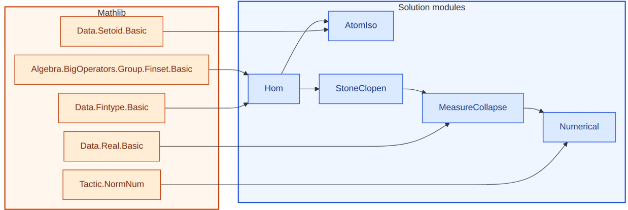
Figure 16: Lean module dependencies for the 21-322 solution. Amber box: Mathlib imports. Blue box: solution modules.
