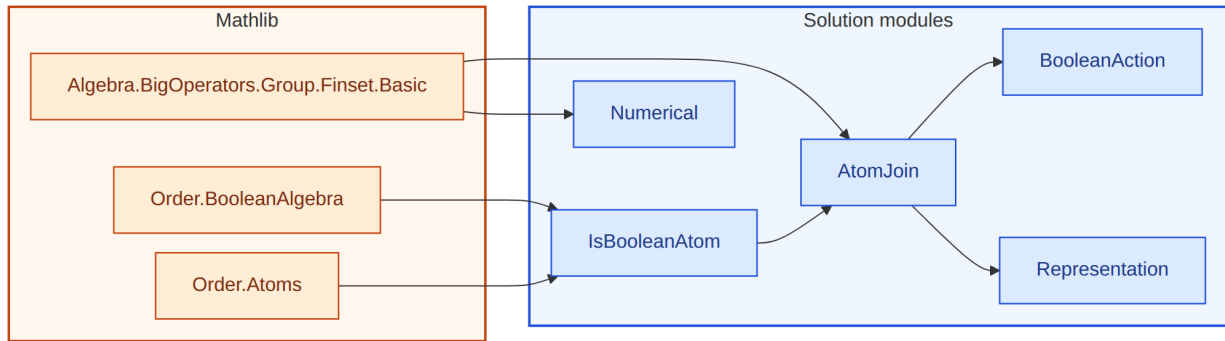
Figure 8: Lean module dependencies for the 21-373 solution. Amber box: Mathlib imports. Blue box: solution modules.
