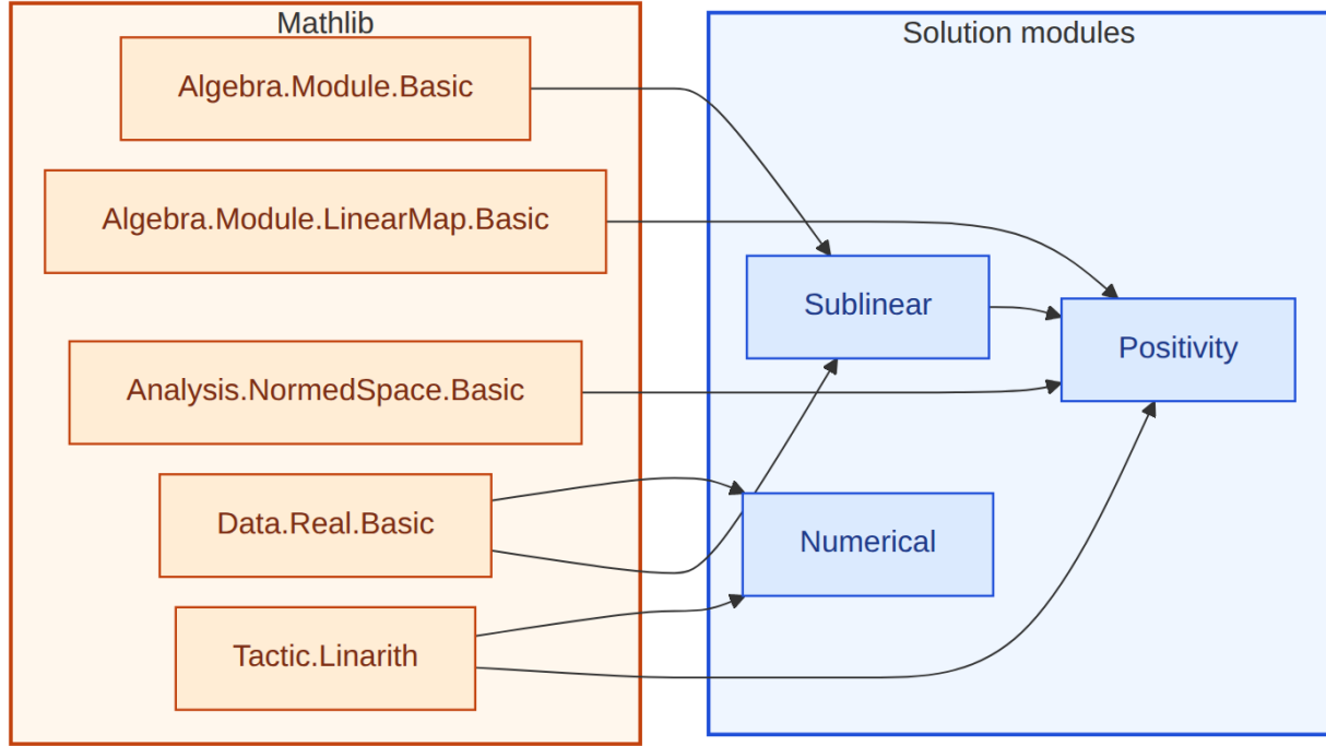
Figure 14: Lean module dependencies for the 21-640 solution. Amber box: Mathlib imports. Blue box: solution modules.
