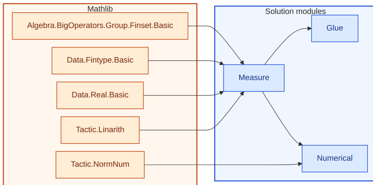
Figure 15: Lean module dependencies for the 21-410 / 21-599 solution. Amber box: Mathlib imports. Blue box: solution modules.
