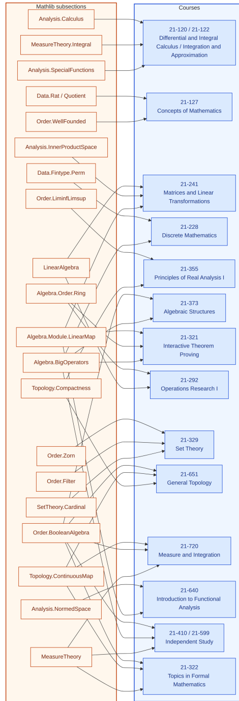
Figure 2: Mathlib subsections required to read each course. Orange nodes are Mathlib; blue nodes are courses. Course nodes are hyperlinked to the corresponding section.
