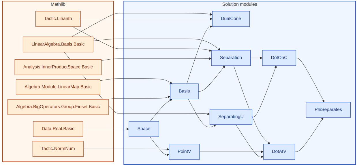
Figure 5: Lean module dependencies for the 21-241 solution. Amber box: Mathlib imports. Blue box: solution modules.
