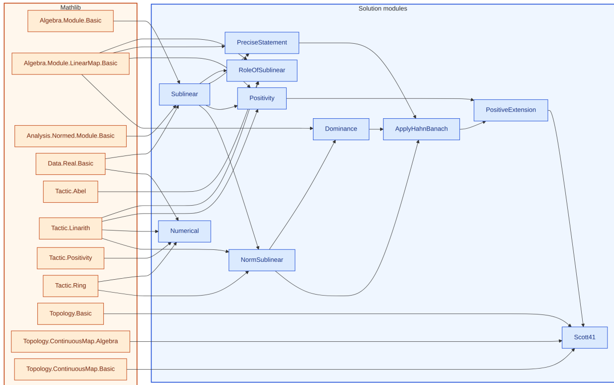
Figure 14: Lean module dependencies for the 21-640 solution. Amber box: Mathlib imports. Blue box: solution modules.
