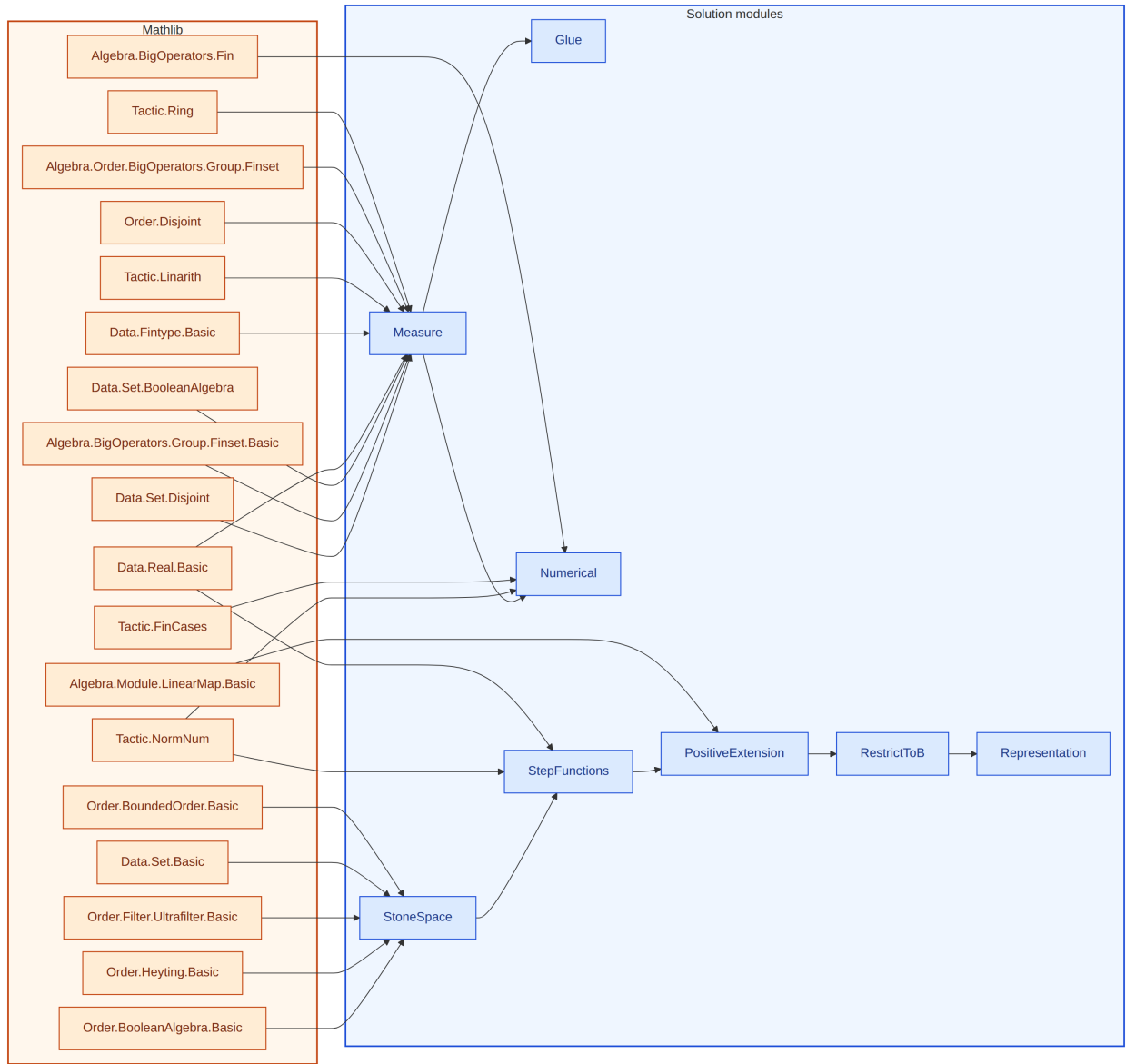
Figure 15: Lean module dependencies for the 21-410 / 21-599 solution. Amber box: Mathlib imports. Blue box: solution modules.
