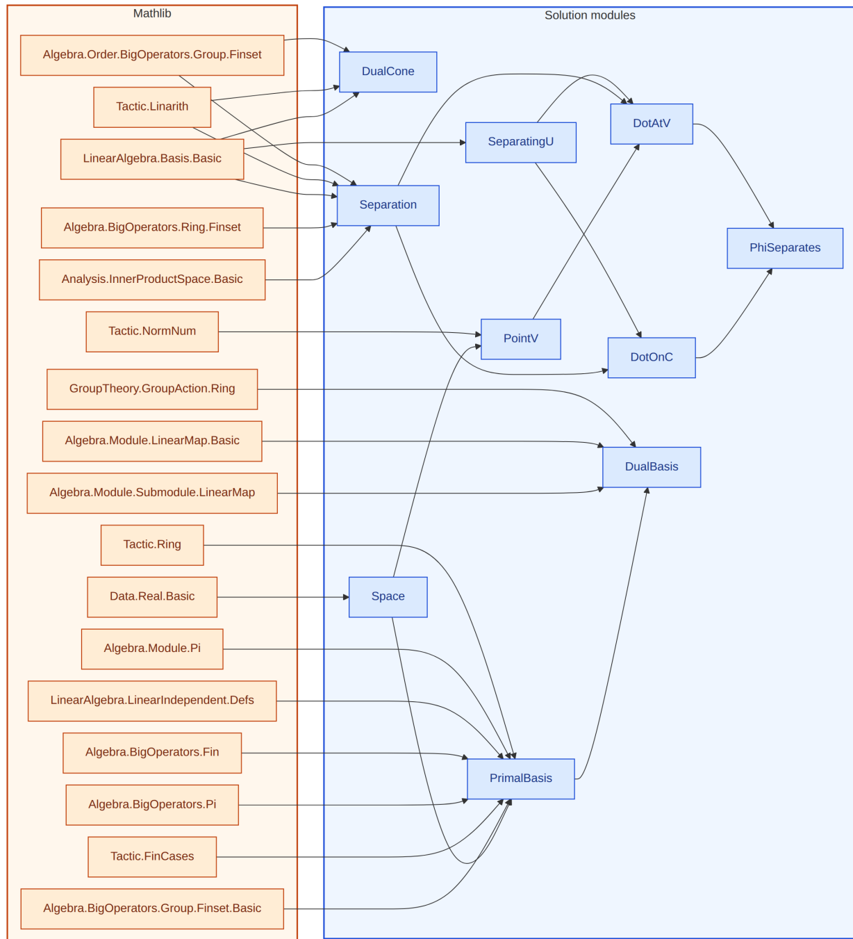
Figure 5: Lean module dependencies for the 21-241 solution. Amber box: Mathlib imports. Blue box: solution modules.
