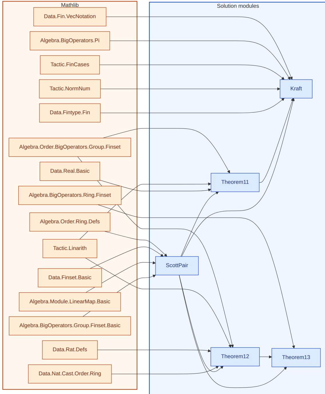
Figure 9: Lean module dependencies for the 21-321 solution. Amber box: Mathlib imports. Blue box: solution modules.
