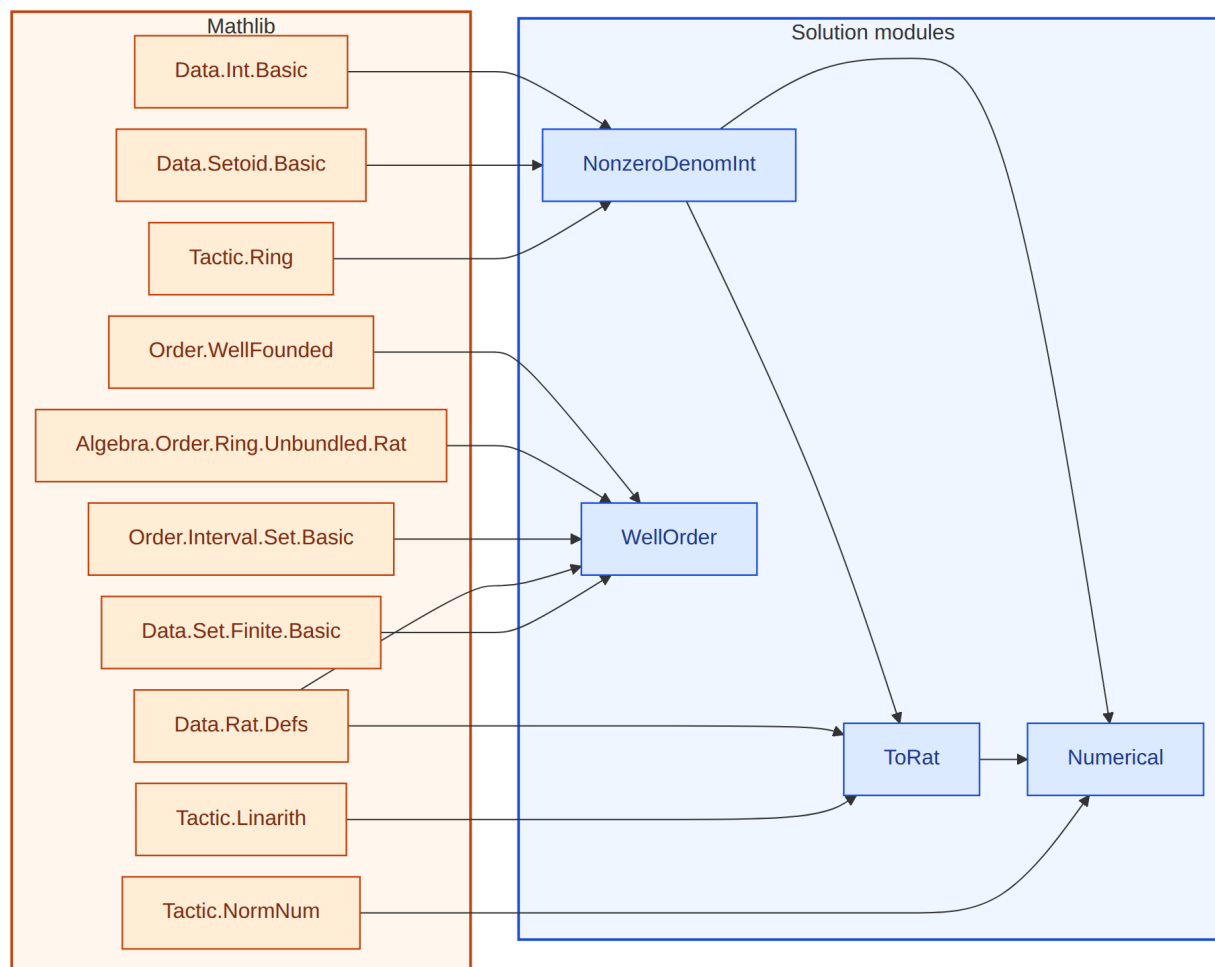
Figure 4: Lean module dependencies for the 21-127 solution. Amber box: Mathlib imports. Blue box: solution modules.
