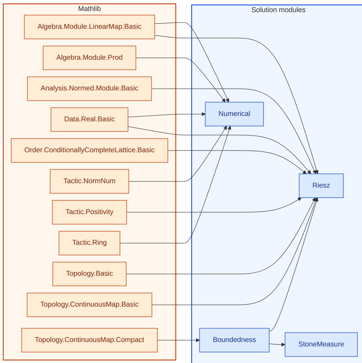
Figure 13: Lean module dependencies for the 21-720 solution. Amber box: Mathlib imports. Blue box: solution modules.
