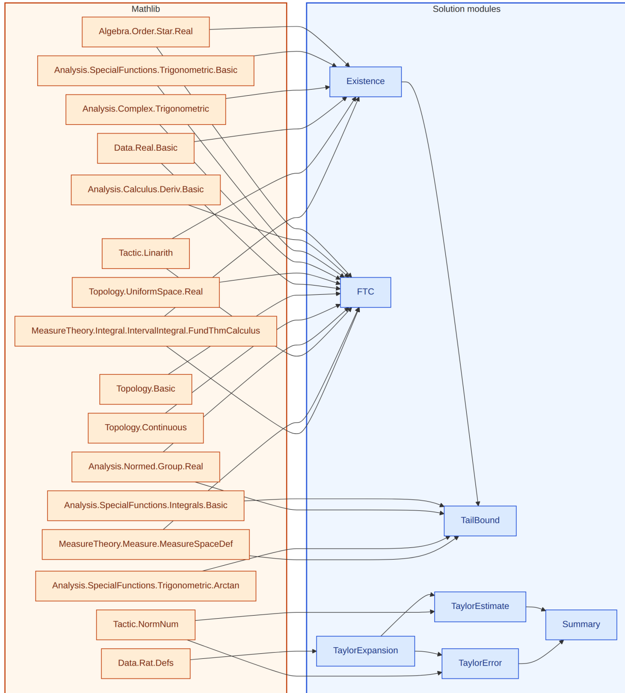
Figure 3: Lean module dependencies for the 21-120 / 21-122 solution. Amber box: Mathlib imports. Blue box: solution modules.
