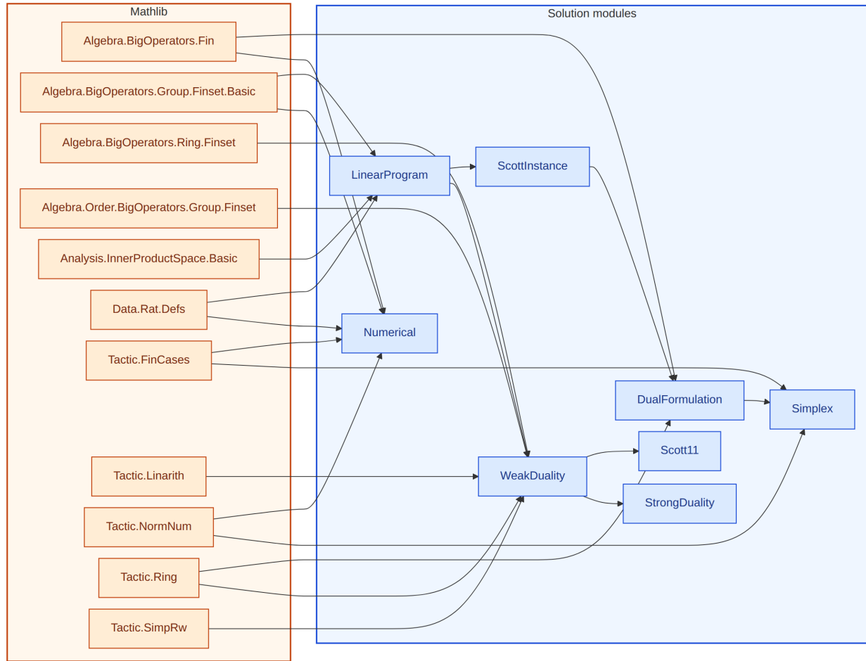
Figure 10: Lean module dependencies for the 21-292 solution. Amber box: Mathlib imports. Blue box: solution modules.
