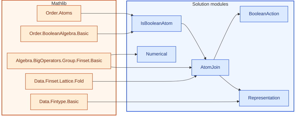
Figure 8: Lean module dependencies for the 21-373 solution. Amber box: Mathlib imports. Blue box: solution modules.
