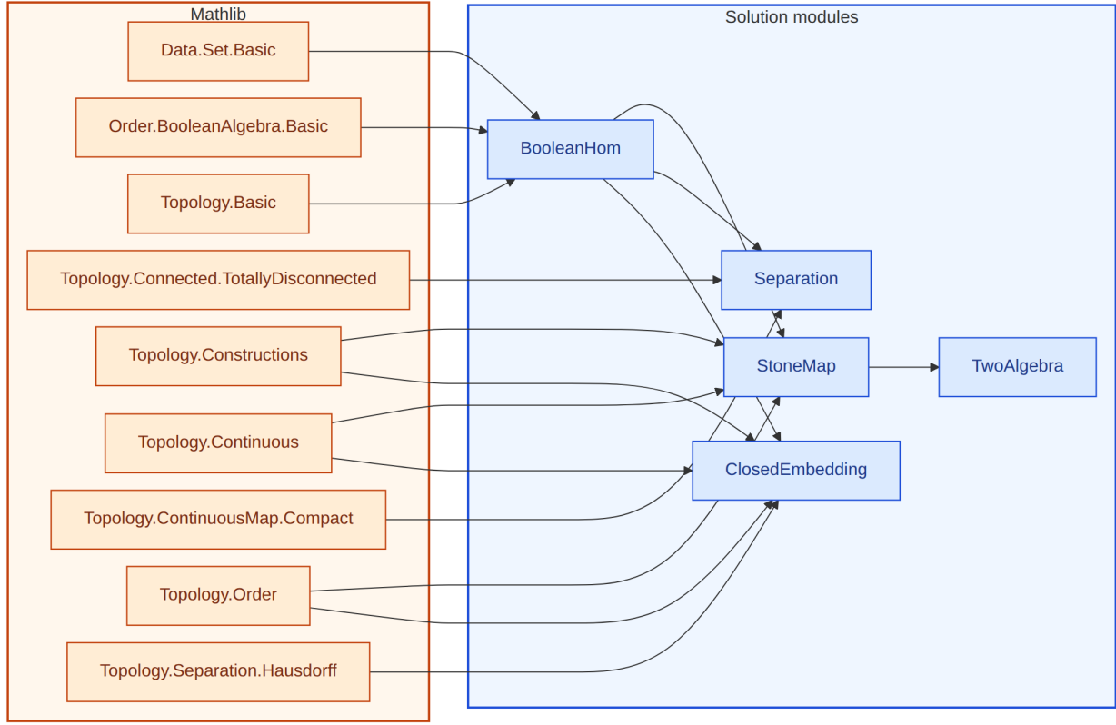
Figure 12: Lean module dependencies for the 21-651 solution. Amber box: Mathlib imports. Blue box: solution modules.
