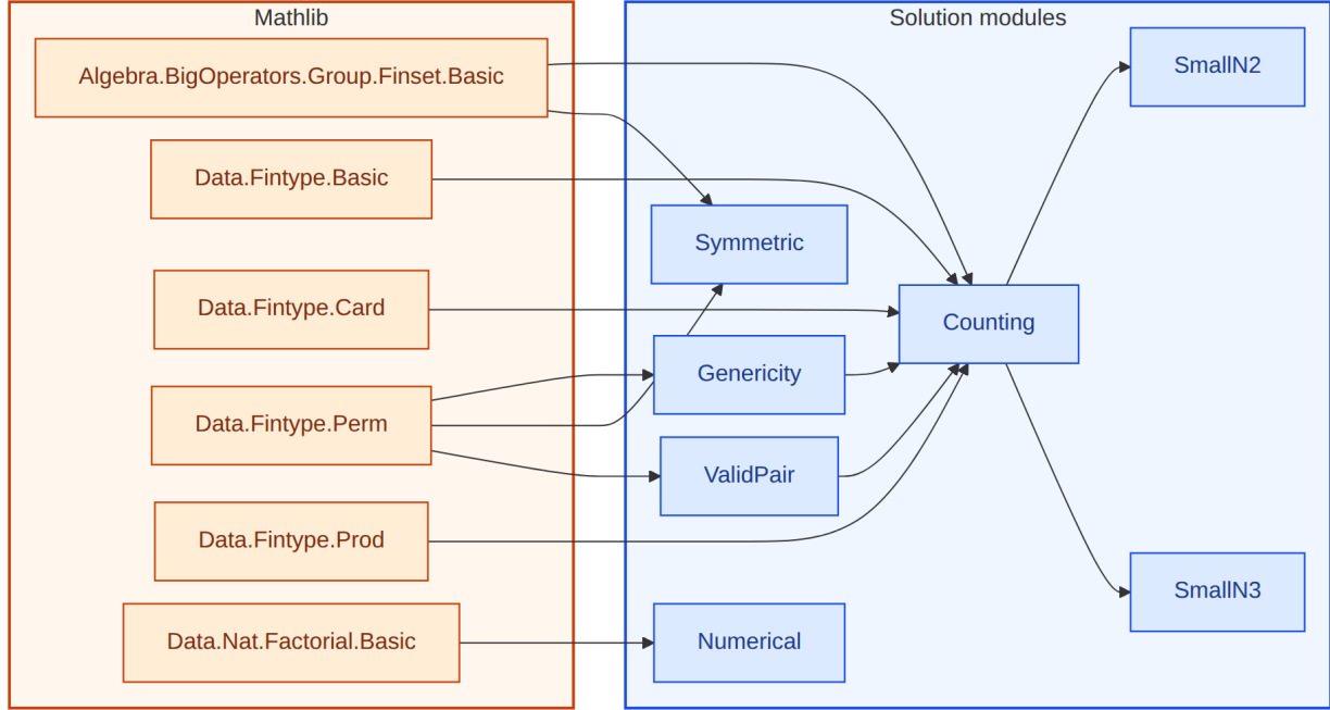
Figure 6: Lean module dependencies for the 21-228 solution. Amber box: Mathlib imports. Blue box: solution modules.
