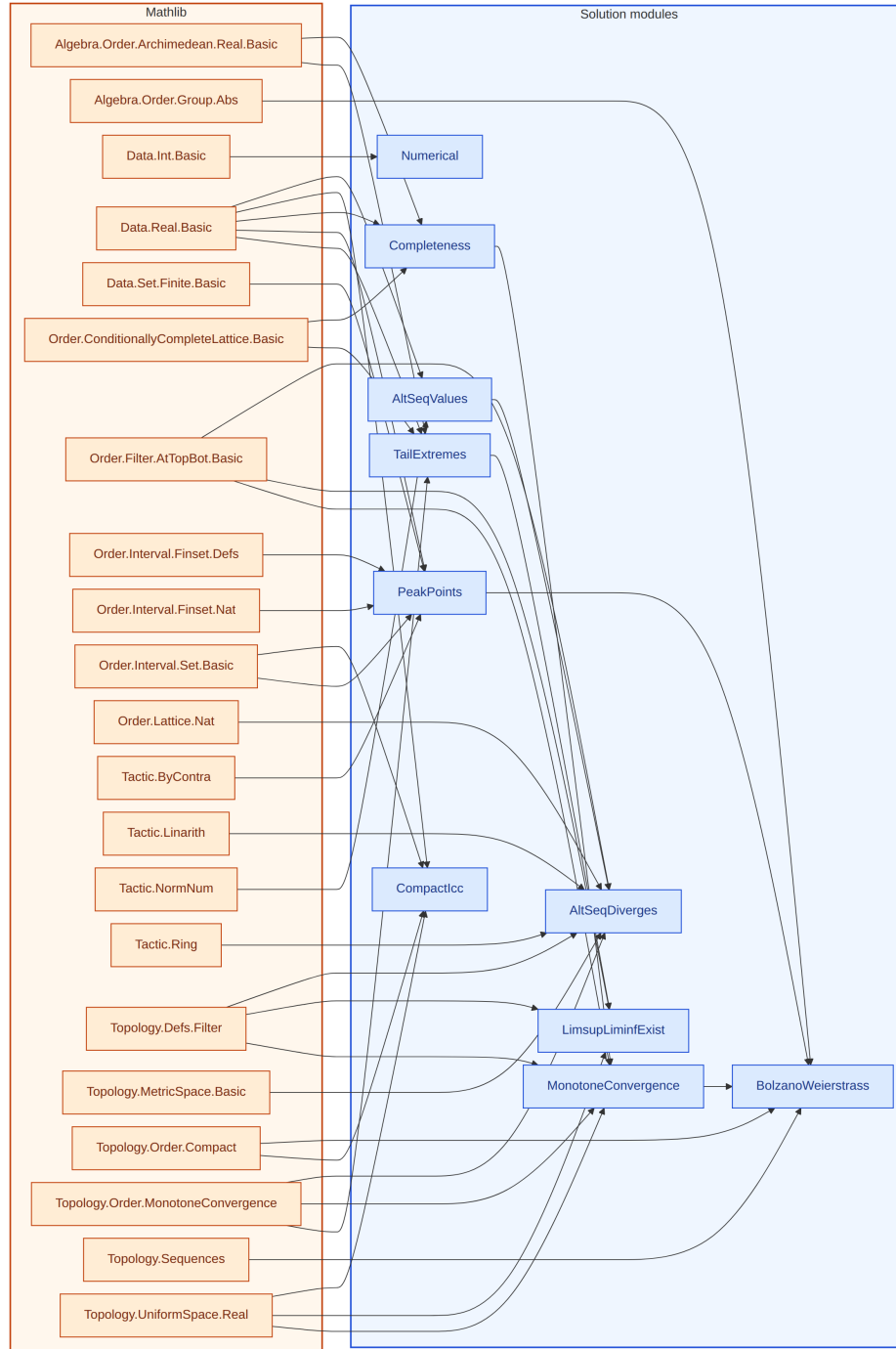
Figure 7: Lean module dependencies for the 21-355 solution. Amber box: Mathlib imports. Blue box: solution modules.
