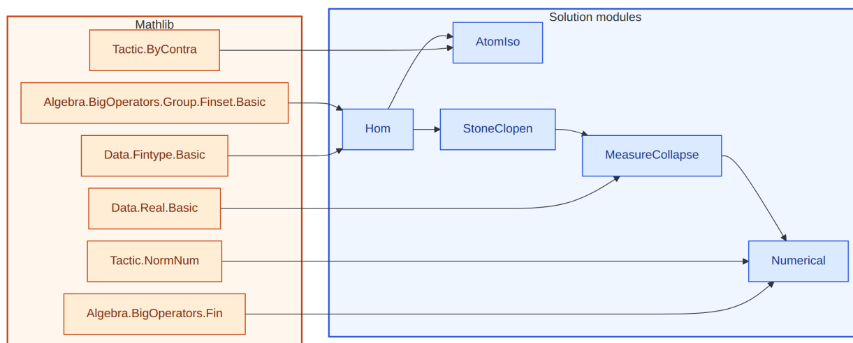
Figure 16: Lean module dependencies for the 21-322 solution. Amber box: Mathlib imports. Blue box: solution modules.
