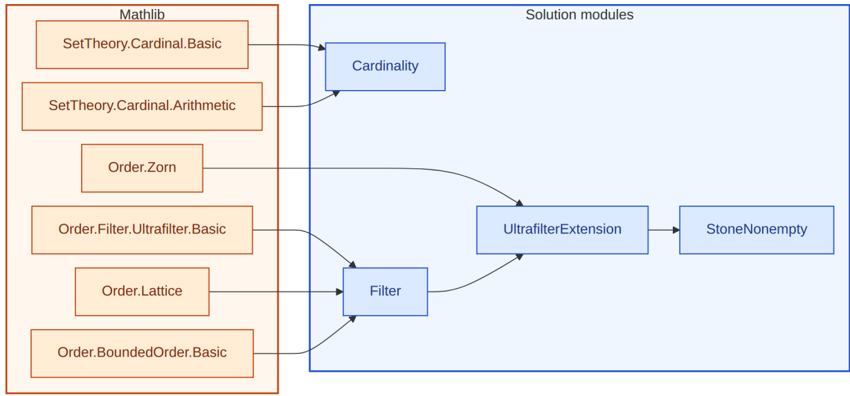
Figure 11: Lean module dependencies for the 21-329 solution. Amber box: Mathlib imports. Blue box: solution modules.
