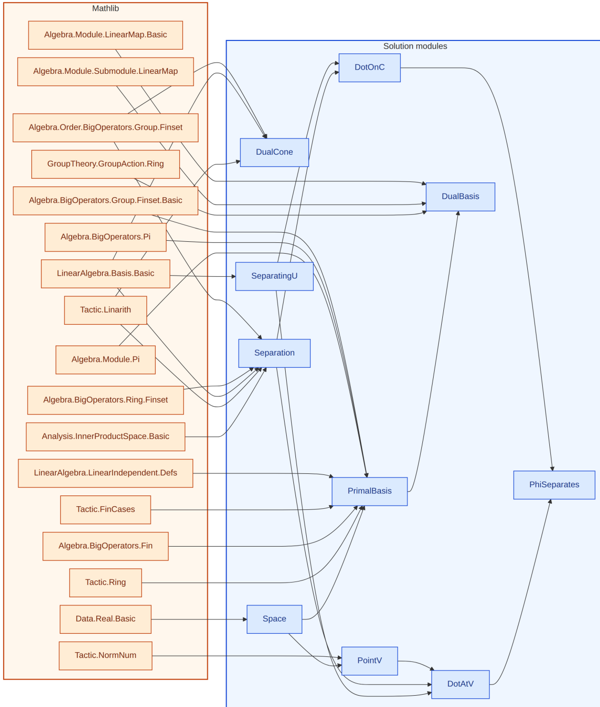
Figure 5: Lean module dependencies for the 21-241 solution. Amber box: Mathlib imports. Blue box: solution modules.
