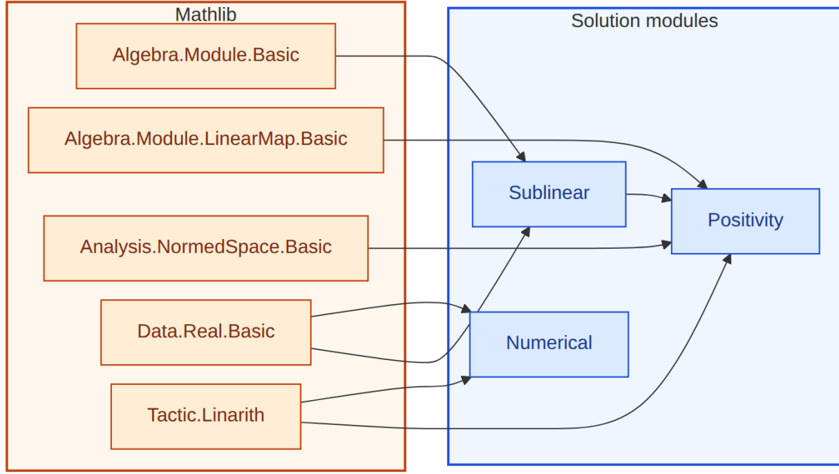
Figure 14: Lean module dependencies for the 21-640 solution. Amber box: Mathlib imports. Blue box: solution modules.
