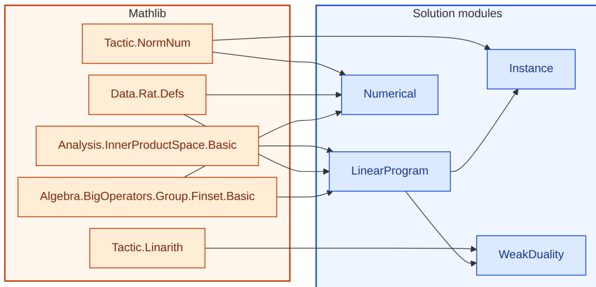
Figure 10: Lean module dependencies for the 21-292 solution. Amber box: Mathlib imports. Blue box: solution modules.
