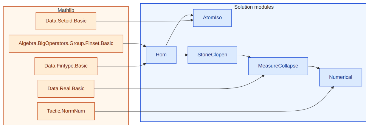
Figure 16: Lean module dependencies for the 21-322 solution. Amber box: Mathlib imports. Blue box: solution modules.
