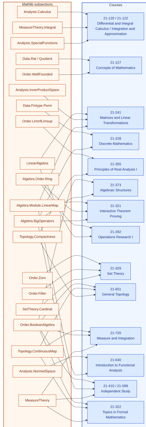
Figure 2: Mathlib subsections required to read each course. Orange nodes are Mathlib; blue nodes are courses.
