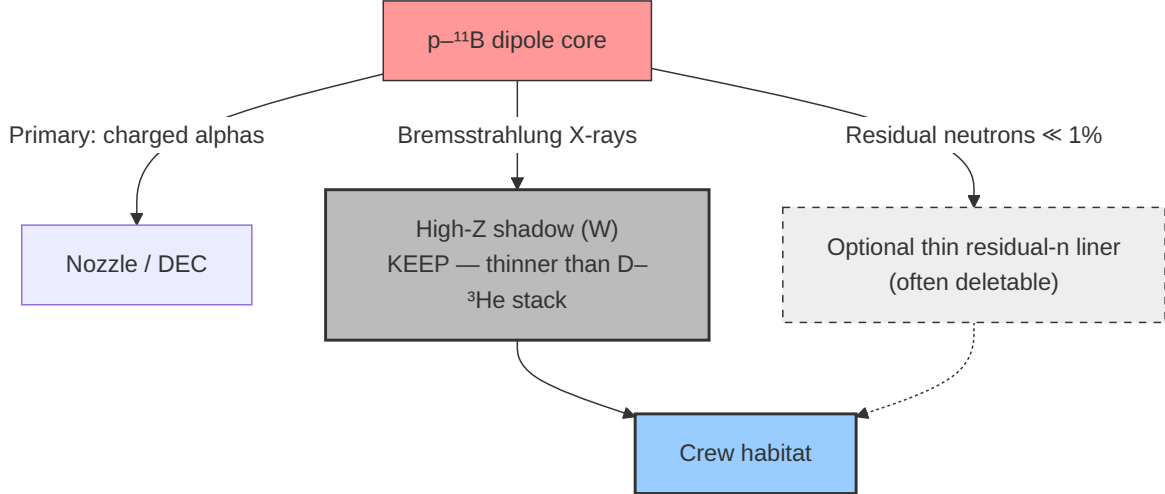
Figure 3 X-ray / Bremsstrahlung shield — keep, possibly thin differently.
