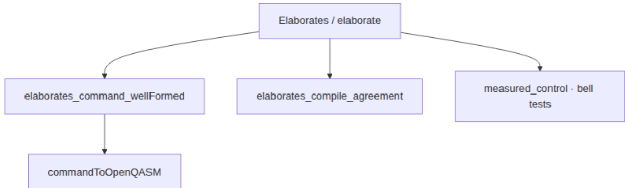
Figure 6: Section 6 theorem dependence: successful elaboration yields
