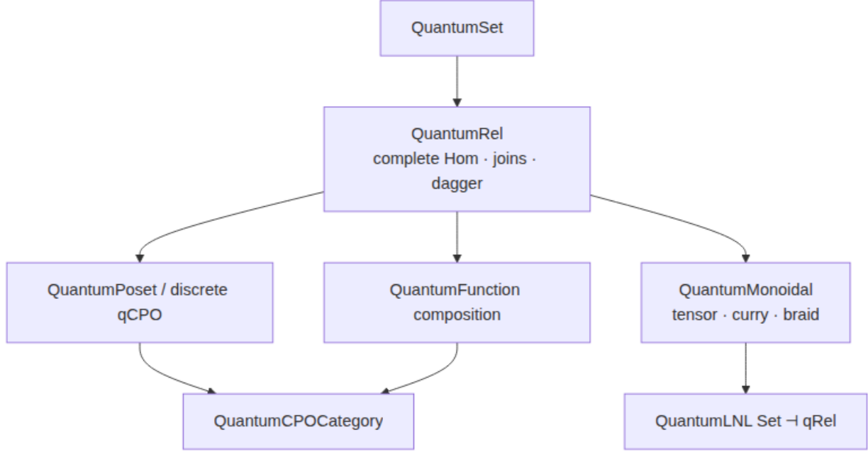
Figure 4: Section 4 theorem dependence: quantum-relation algebra supports the
