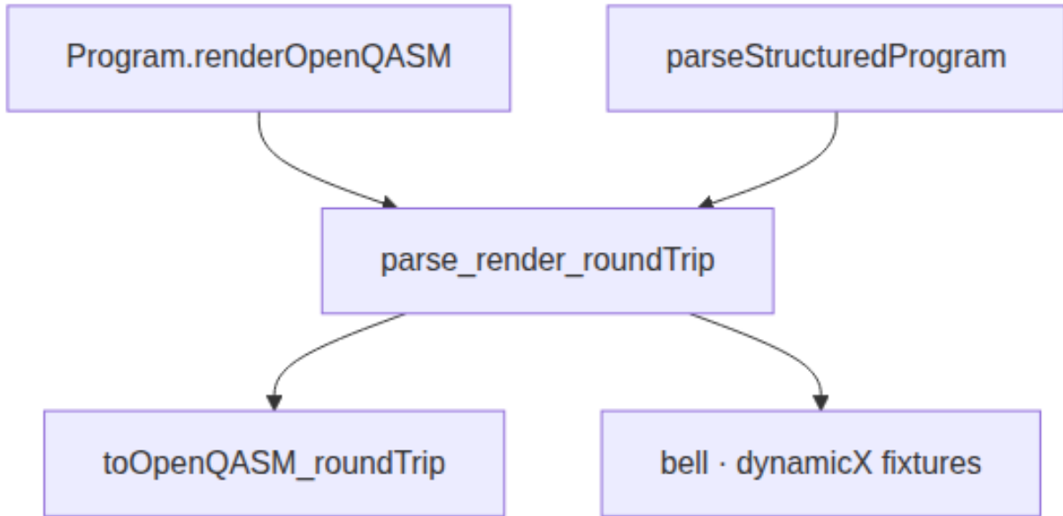
Figure 8: Section 8 theorem dependence: canonical OpenQASM render/parse
