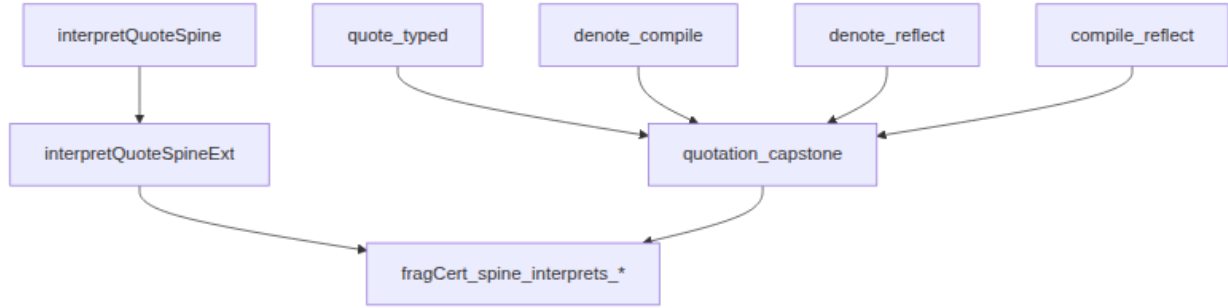
Figure 7: Section 7 theorem dependence: two-wire quotation capstone and the
