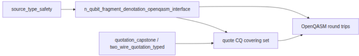
Figure 9: Section 9 claim-surface dependence among the Palomar-facing and
