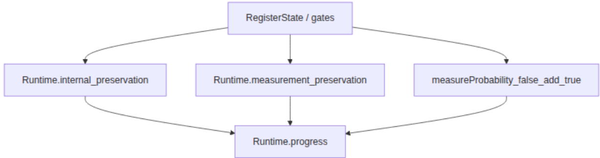
Figure 3: Section 3 theorem dependence: register dynamics support internal
