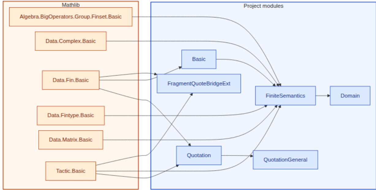
Figure 13: Lean module dependencies for §7 (quotation and completeness). Amber box: Mathlib imports (6 listed). Blue box: project modules (6).
