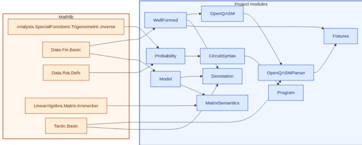
Figure 15: Lean module dependencies for §8 (Composer / OpenQASM). Amber box: Mathlib imports (5 listed). Blue box: project modules (10).
