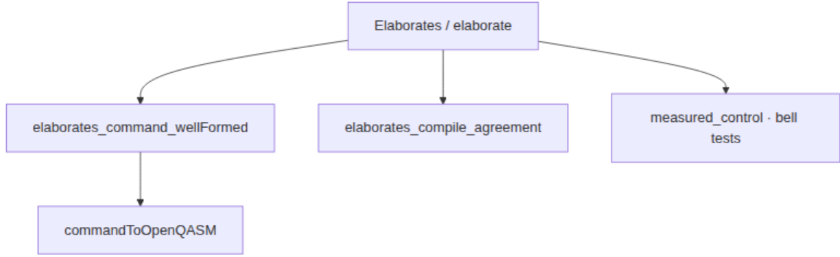
Figure 10: Section 6 theorem dependence: successful elaboration yields
