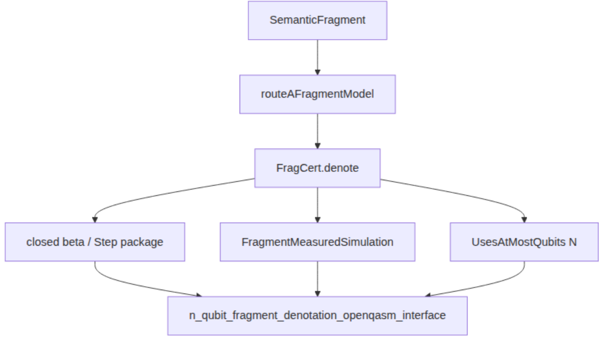
Figure 8: Section 5 checked-fragment theorem dependence culminating in the
