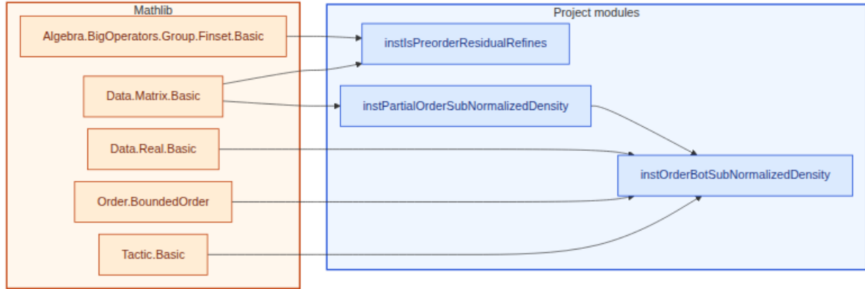
Figure 17: Lean module dependencies for §9 (supporting primitives). Amber box: Mathlib imports (5 listed). Blue box: project modules (3).
