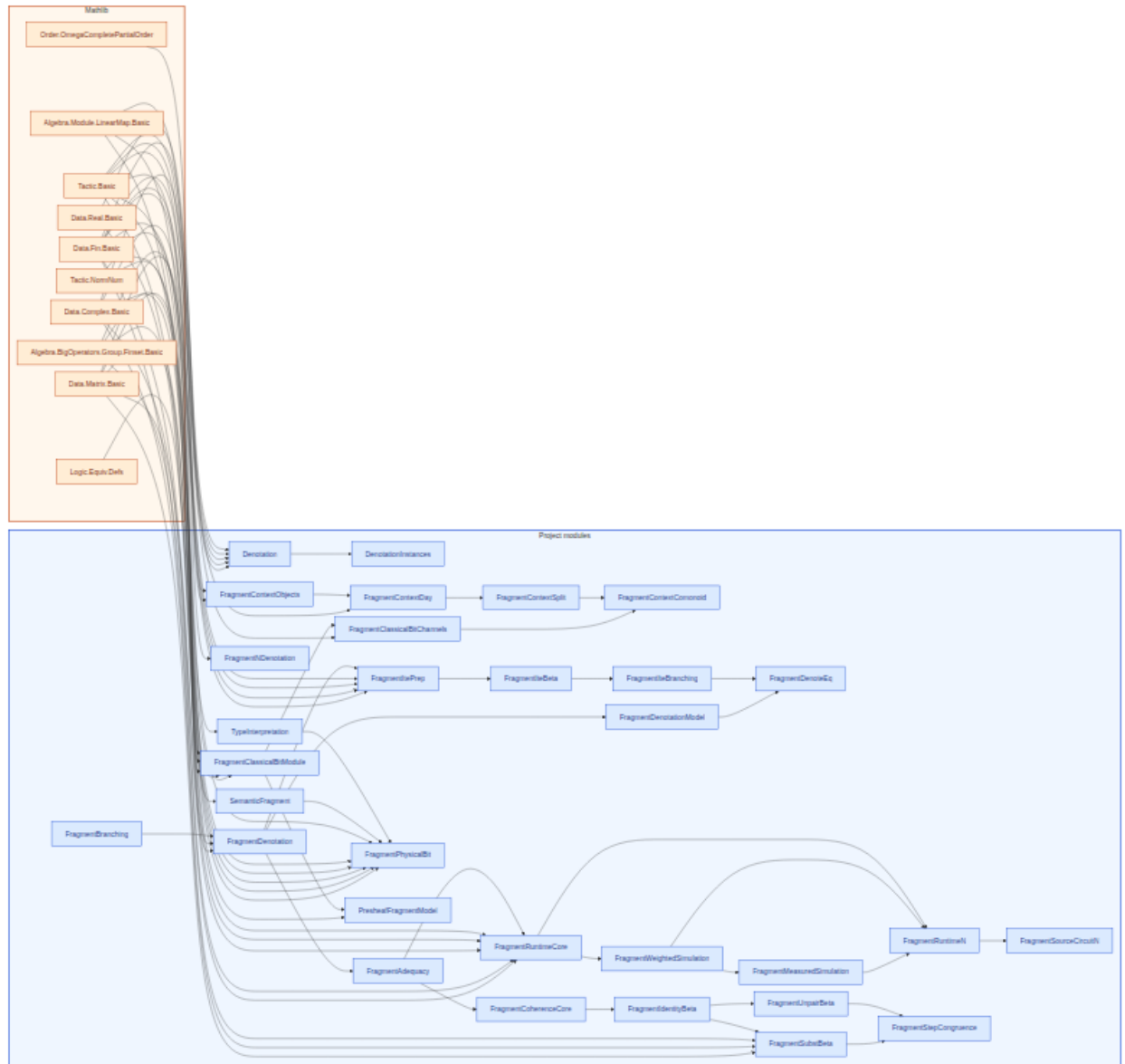
Figure 9: Lean module dependencies for §5 (fragment denotation). Amber box: Mathlib imports (10 listed). Blue box: project modules (31).
