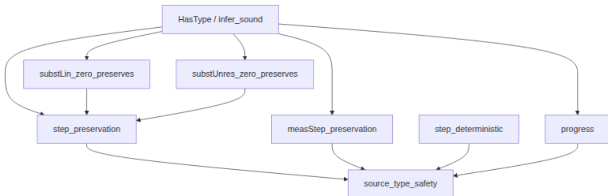
Figure 2: Section 2 theorem dependence: typing and substitution support
