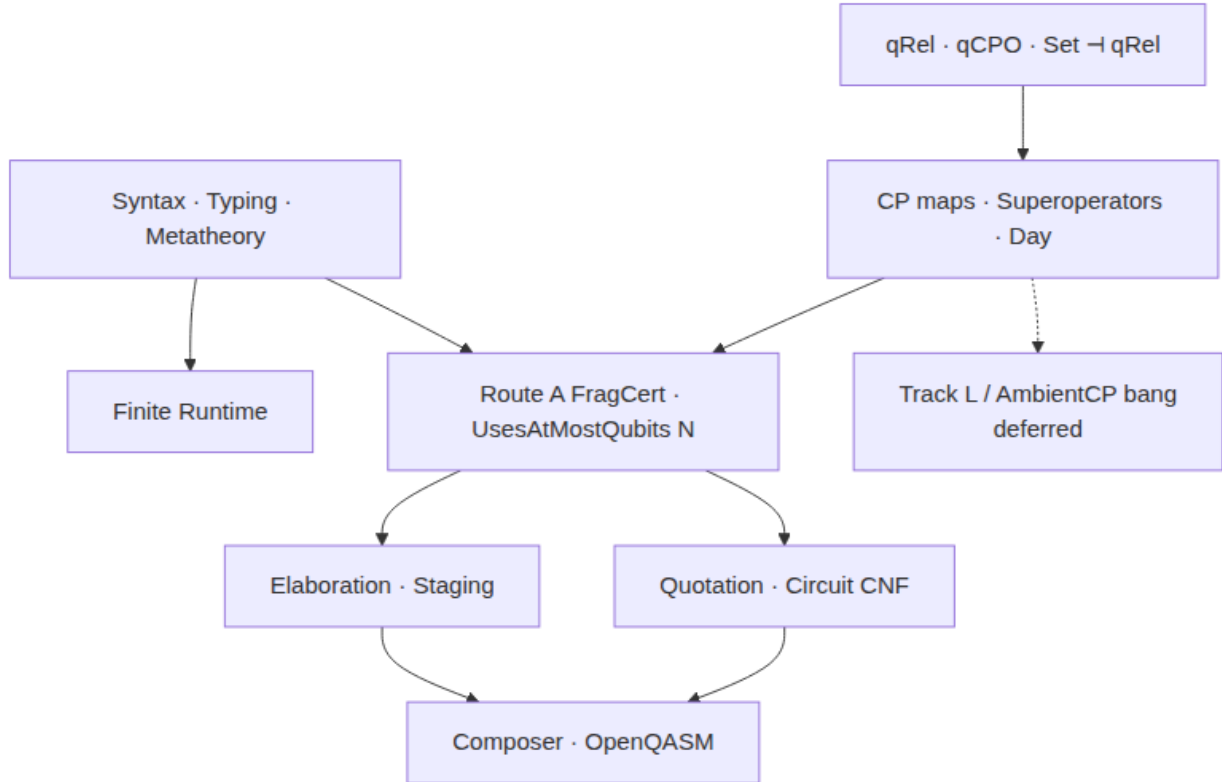
Figure 1: Layered Lean development: checked N -bounded fragment path (solid)
