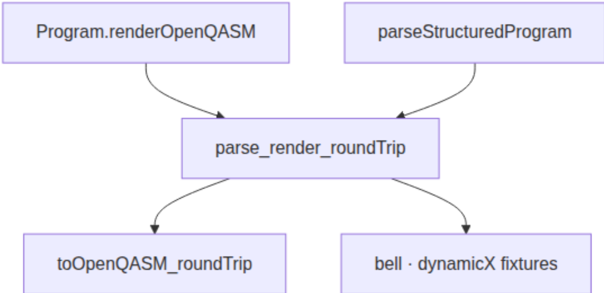
Figure 14: Section 8 theorem dependence: canonical OpenQASM render/parse
