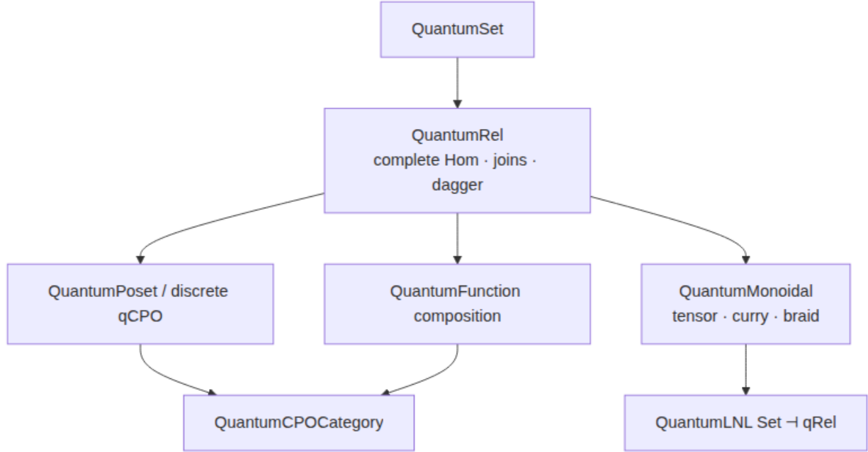
Figure 6: Section 4 theorem dependence: quantum-relation algebra supports the
