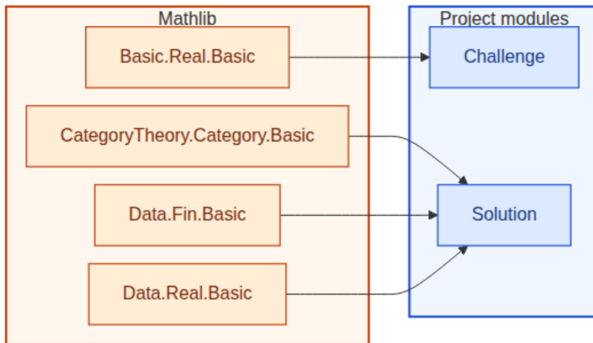
Figure 18: Lean module dependencies for Palomar challenge / solution. Amber box: Mathlib imports (4 listed). Blue box: project modules (2).
