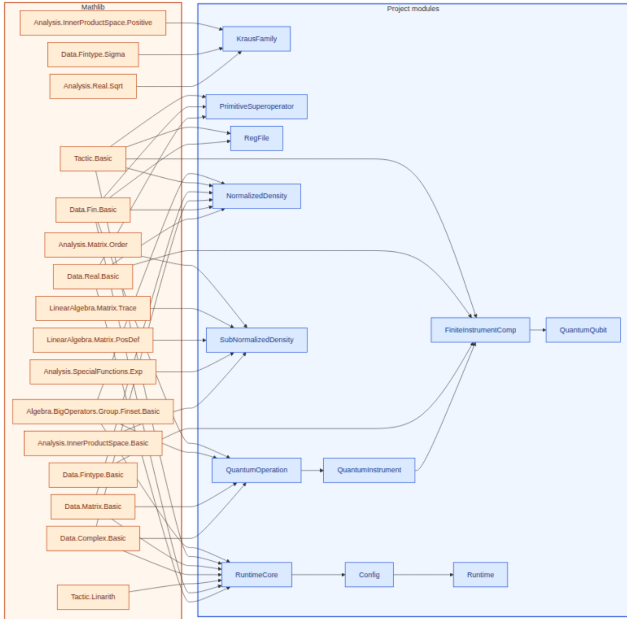
Figure 5: Lean module dependencies for §3 (finite quantum runtime). Amber box: Mathlib imports (16 listed). Blue box: project modules (12).
