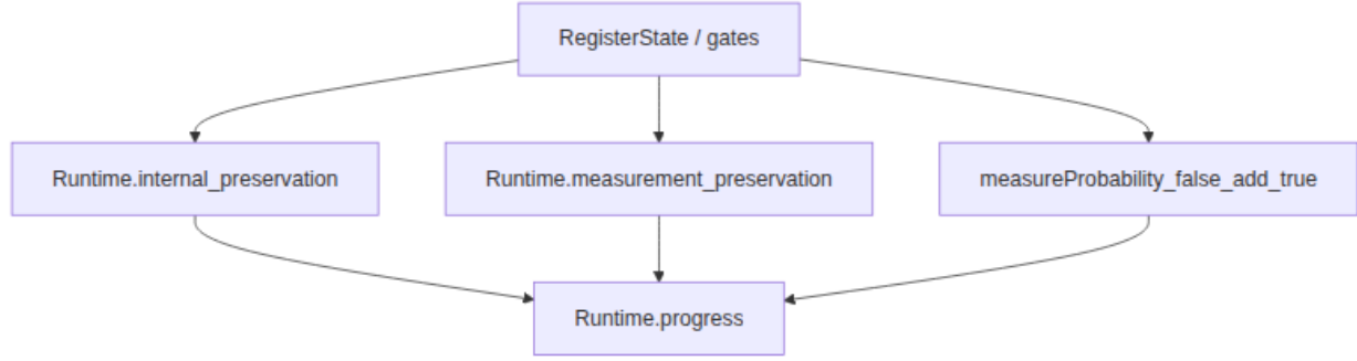
Figure 4: Section 3 theorem dependence: register dynamics support internal
