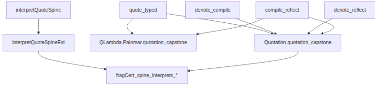
Figure 12: Section 7 theorem dependence. Quotation.quotation_capstone
