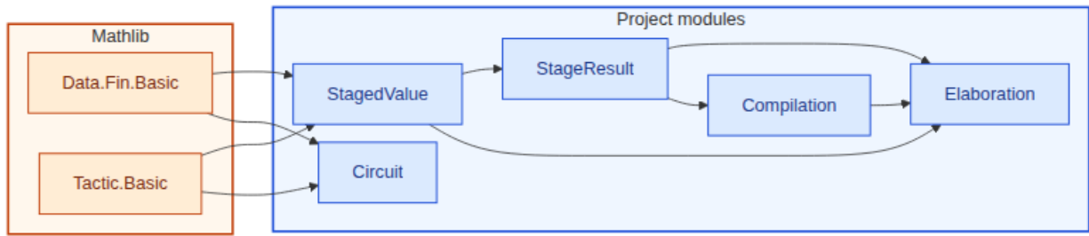
Figure 11: Lean module dependencies for §6 (staging to circuits). Amber box: Mathlib imports (2 listed). Blue box: project modules (5).
