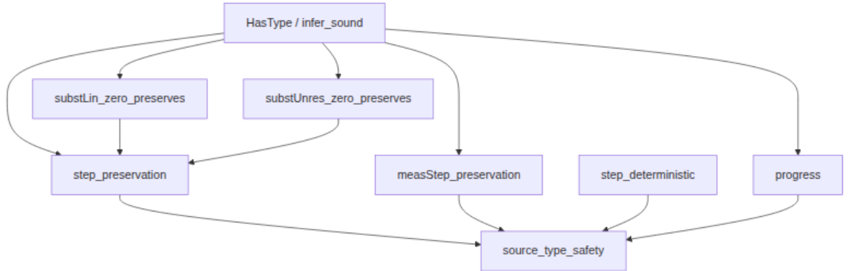
Figure 2: Section 2 theorem dependence: typing and substitution support
