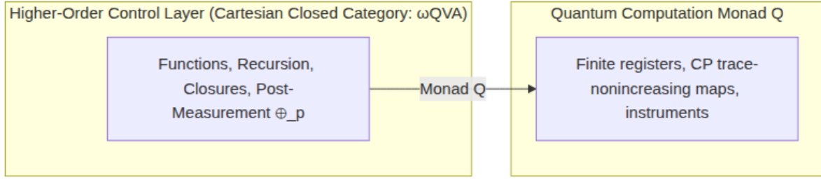
Figure 6: Linear-nonlinear architecture: higher-order classical control in \omega\mathbf{QVA} and the quantum computation monad Q .
