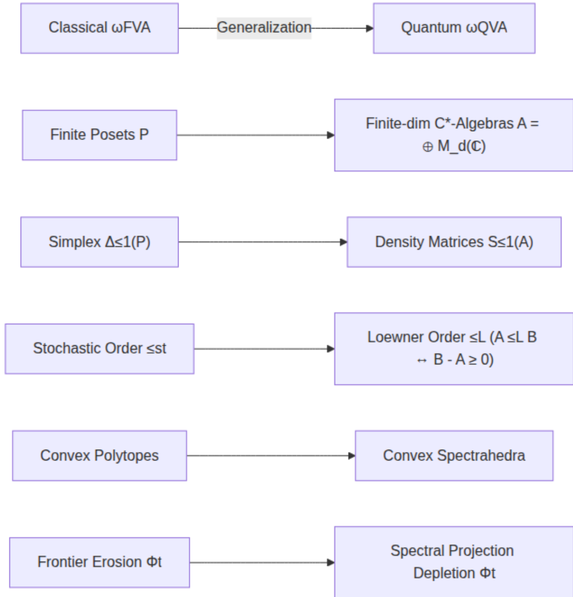
Figure 7: Generalization of Chen–Kou–Lyu \omega\mathbf{FVA} ingredients to spectrahedral \omega\mathbf{QVA} .
