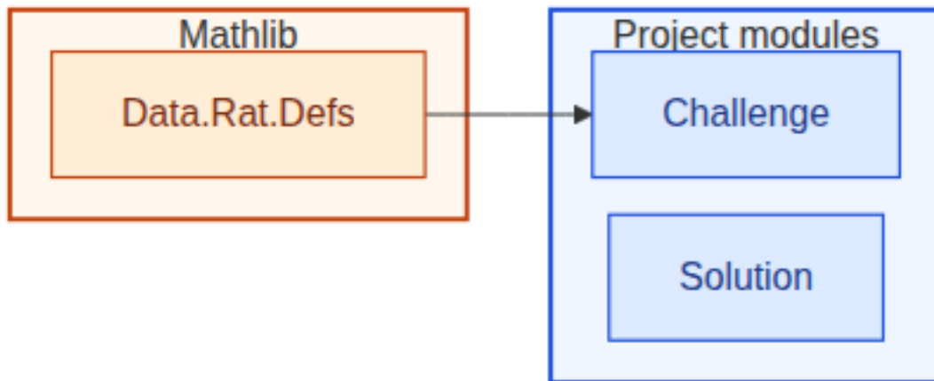
Figure 18: Lean module dependencies for Palomar challenge / solution. Amber box: Mathlib imports (1 listed). Blue box: project modules (2).
