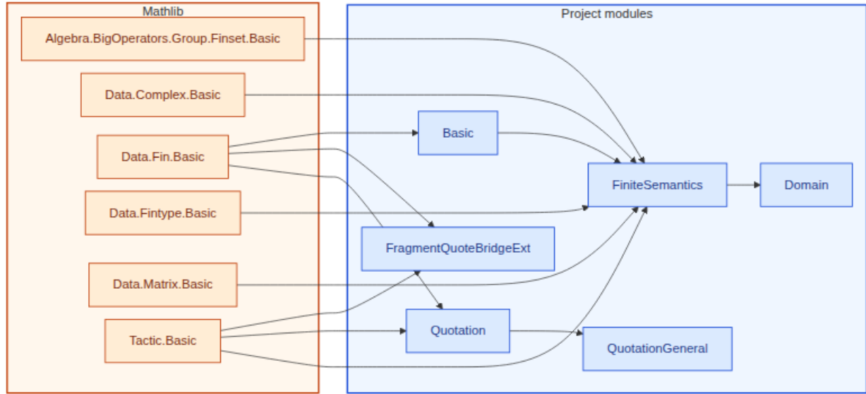
Figure 13: Lean module dependencies for §7 (quotation and completeness). Amber box: Mathlib imports (6 listed). Blue box: project modules (6).
