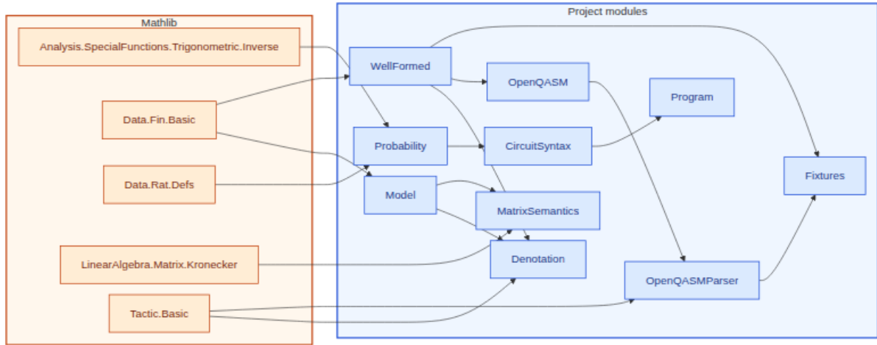
Figure 15: Lean module dependencies for §8 (Composer / OpenQASM). Amber box: Mathlib imports (5 listed). Blue box: project modules (10).
