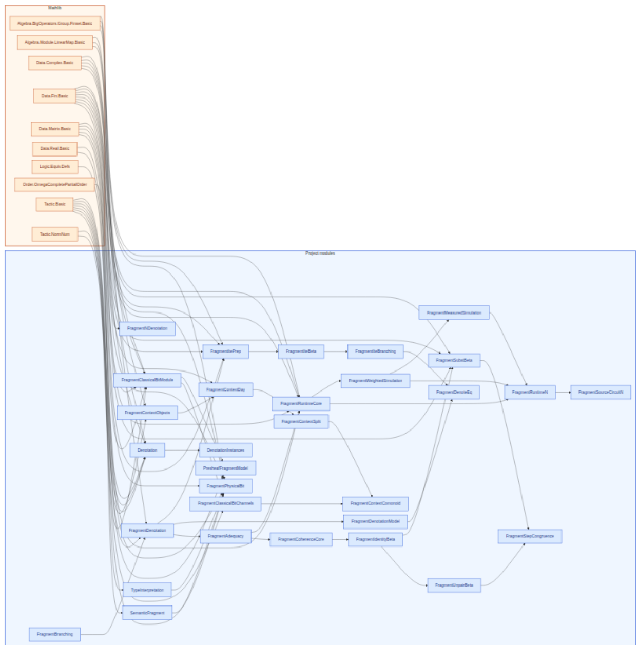
Figure 9: Lean module dependencies for §5 (fragment denotation). Amber box: Mathlib imports (10 listed). Blue box: project modules (31).
