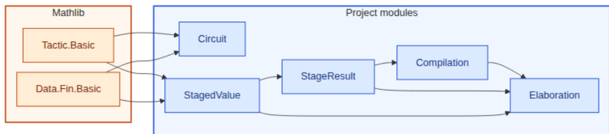
Figure 11: Lean module dependencies for §6 (staging to circuits). Amber box: Mathlib imports (2 listed). Blue box: project modules (5).
