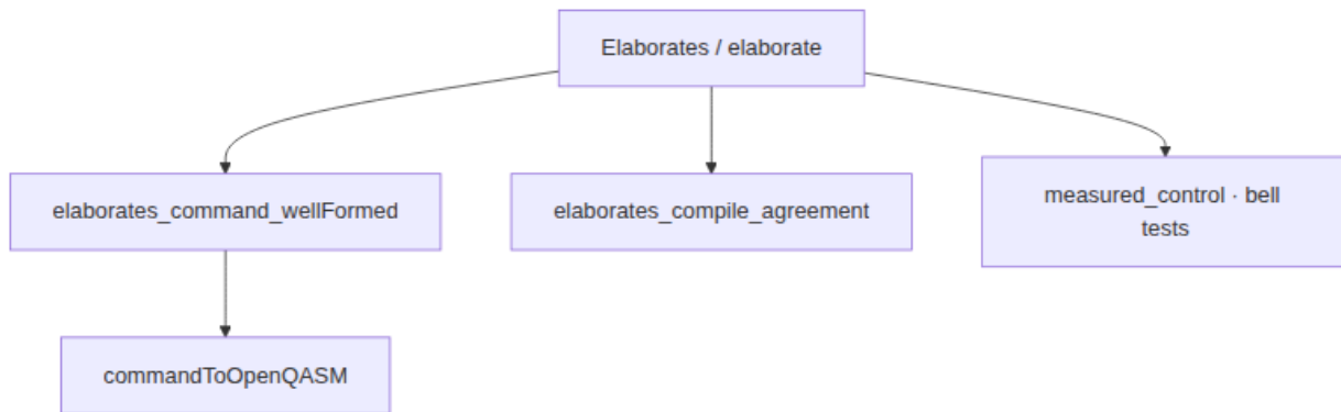
Figure 10: Section 6 theorem dependence: successful elaboration yields
