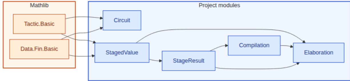
Figure 11: Lean module dependencies for §6 (staging to circuits). Amber box: Mathlib imports (2 listed). Blue box: project modules (5).
