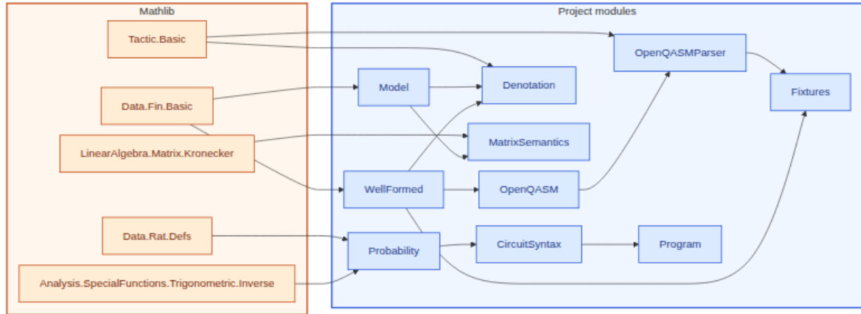
Figure 15: Lean module dependencies for §8 (Composer / OpenQASM). Amber box: Mathlib imports (5 listed). Blue box: project modules (10).
