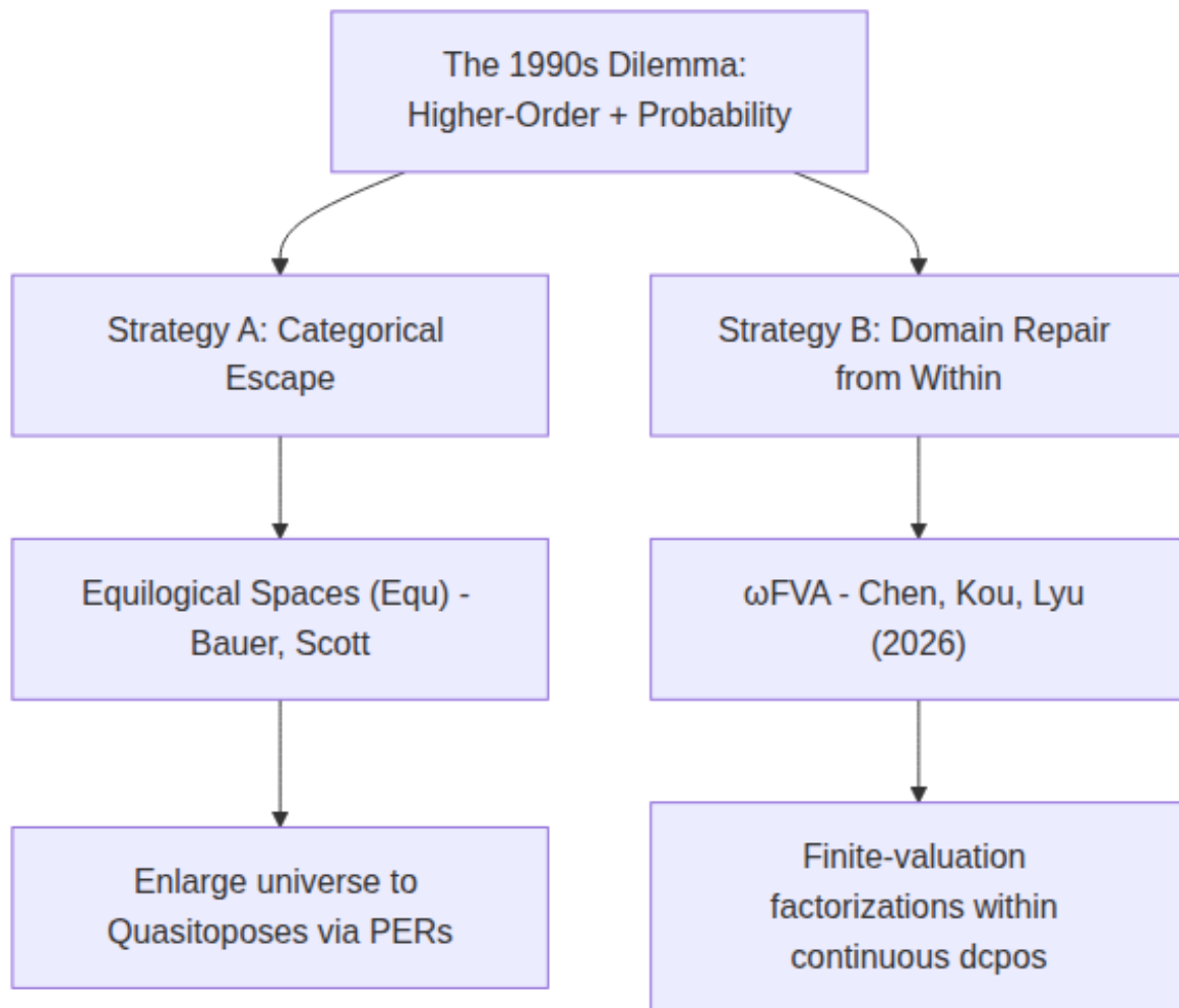
Figure 5: Two historical strategies for combining higher-order functions with probability: equilogical spaces versus \omega\mathbf{FVA} .
