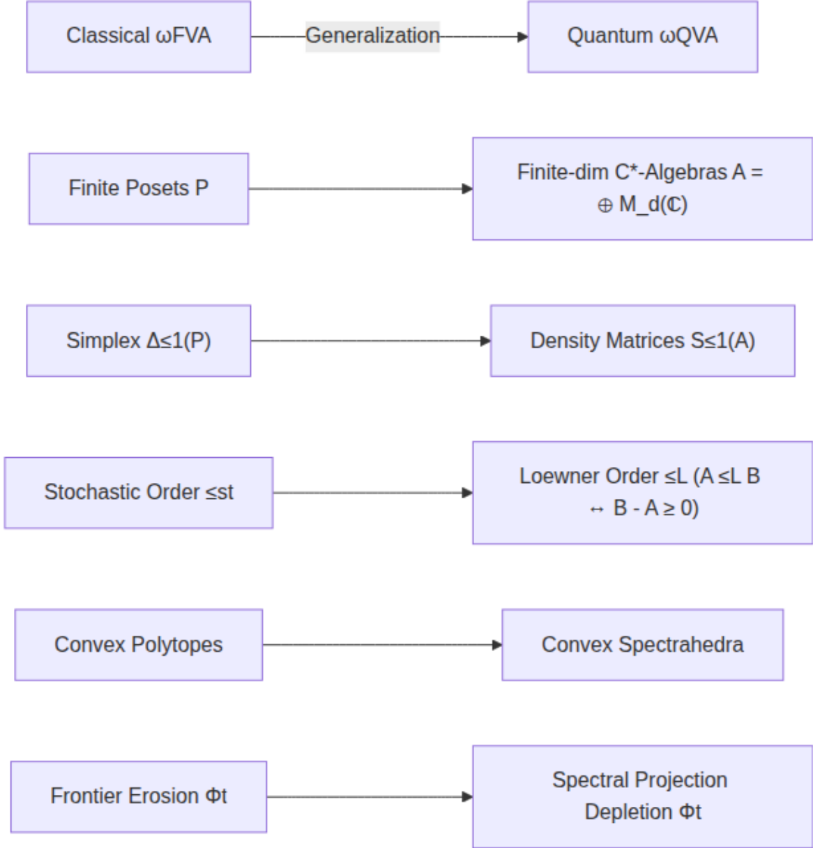
Figure 7: Generalization of Chen–Kou–Lyu \omega FVA ingredients to spectrahedral \omega QVA.
