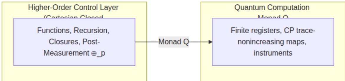
Figure 6: Linear-nonlinear architecture: higher-order classical control in \omega QVA and the quantum computation monad Q .
