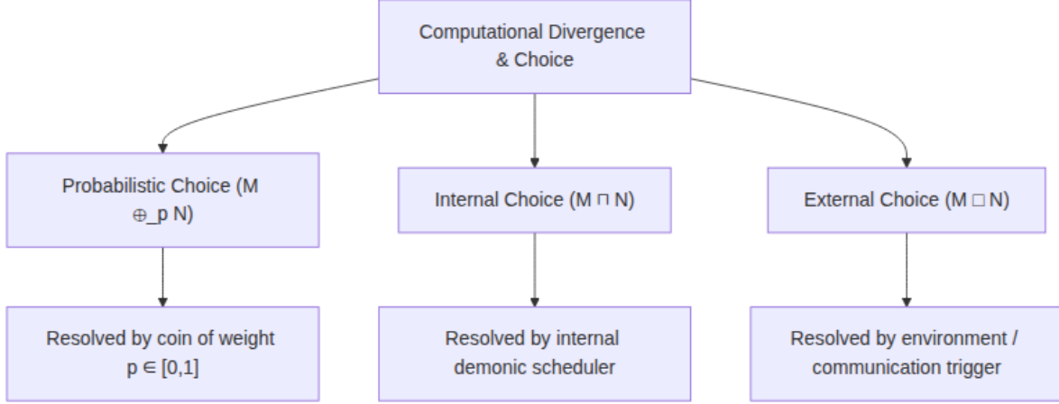
Figure 1: The three classical choice operators and how each is resolved: probabilistic \oplus_p , internal \sqcap , and external \sqbox .
