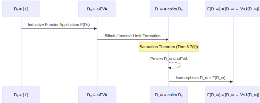
Figure 4: Smyth–Plotkin embedding-projection construction of the bilimit D_\infty in \omega\mathbf{FVA} .
