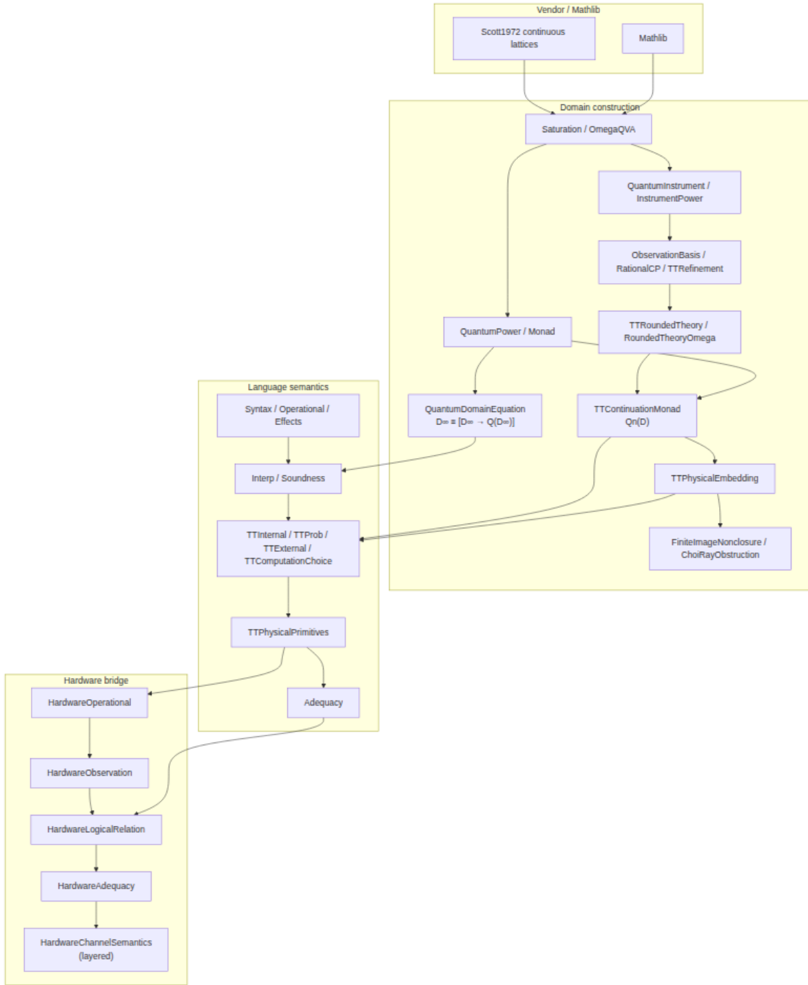
Figure 2: Dependency map of the main Lean modules, from vendored Scott lattices through the domain equation, language semantics, and hardware channel-tree layer.
