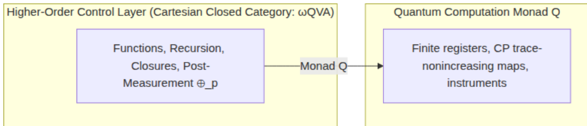
Figure 6: Linear-nonlinear architecture: higher-order classical control in \omega QVA and the quantum computation monad Q .
