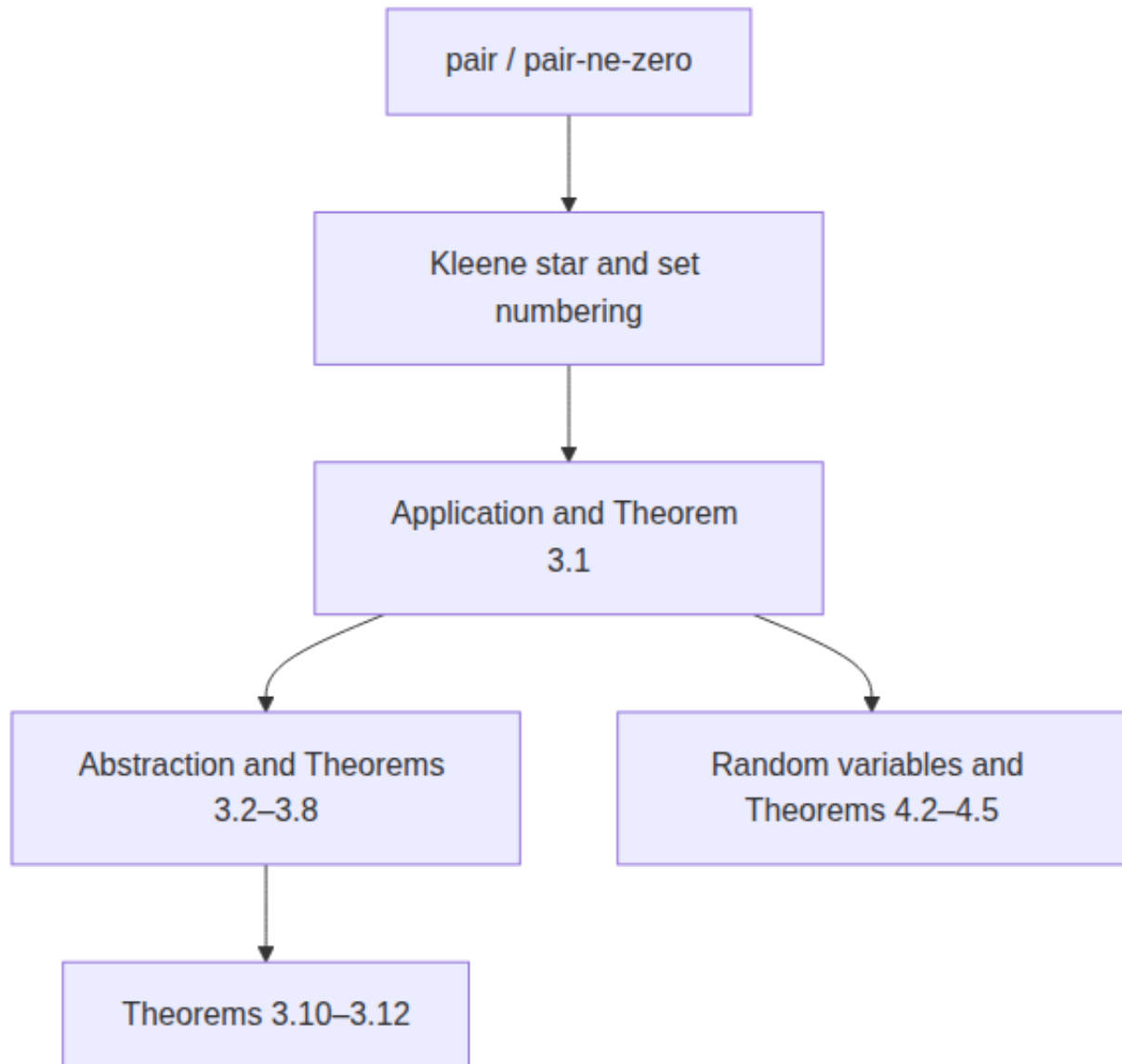
Figure 1: Intended library layers: encodings, graph-model \lambda -calculus, then random variables.
