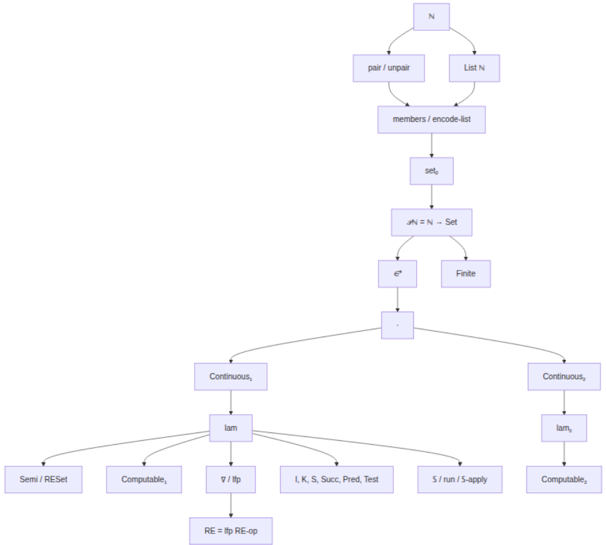
Figure 1: Graph-model encodings and operator types.
