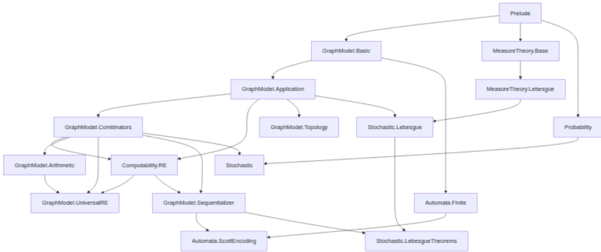
Figure 7: Implemented Agda module imports.
