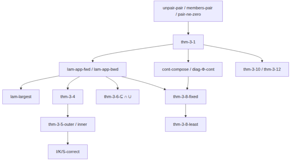
Figure 4: Graph-model proof dependencies through Theorem 3.8.
