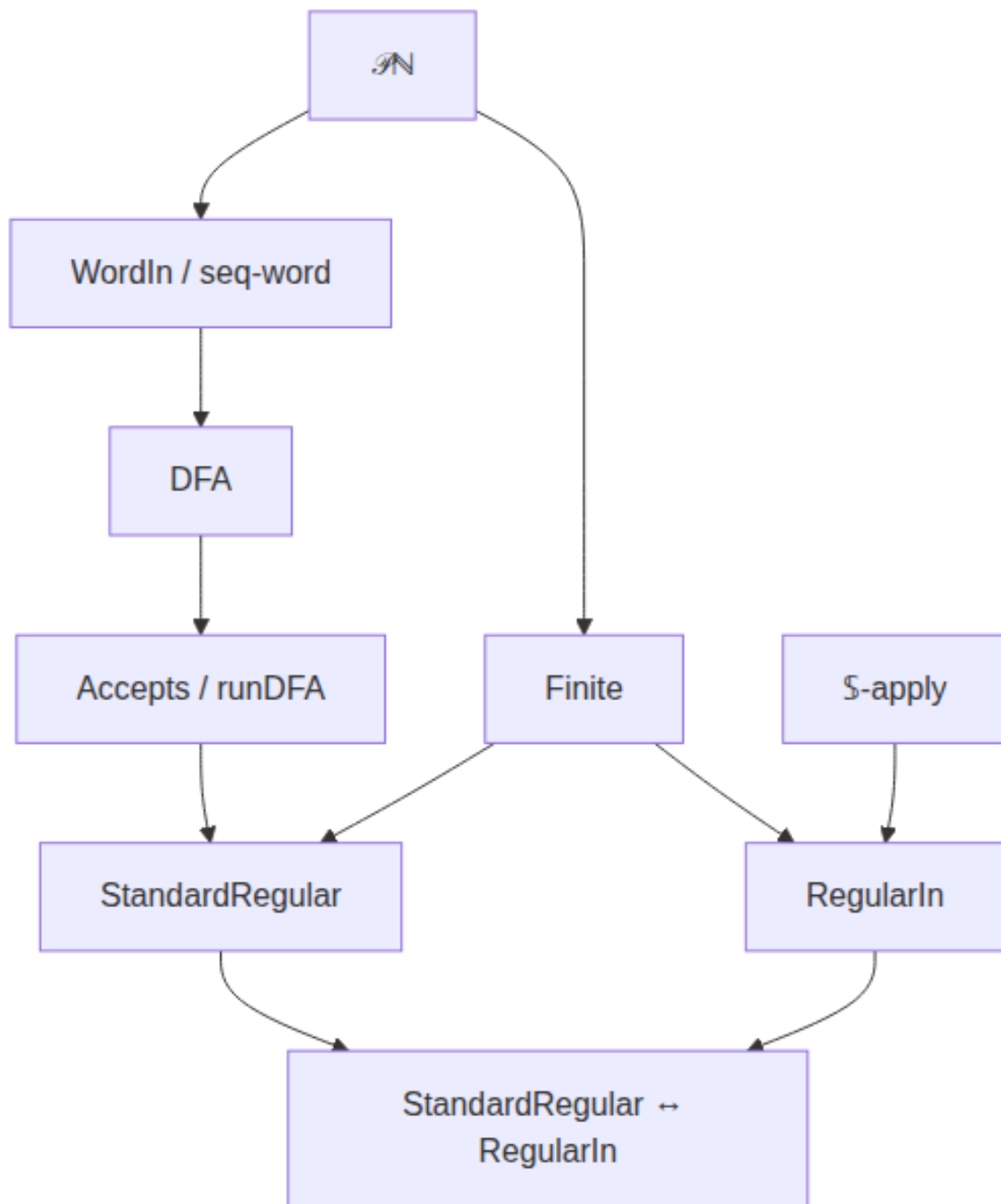
Figure 2: Language and automaton types.
