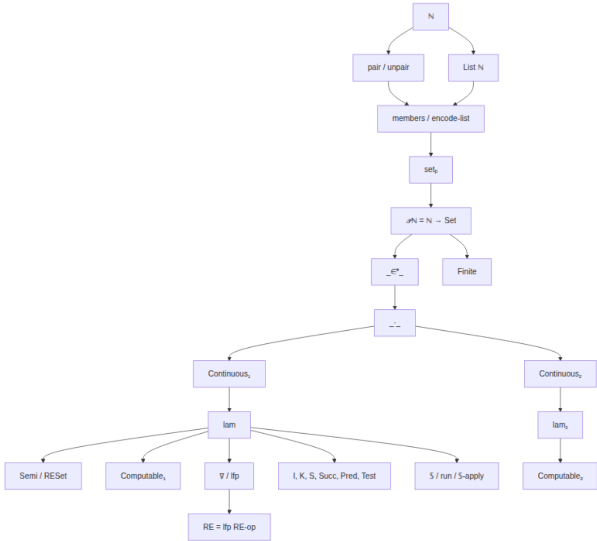
Figure 1: Graph-model encodings and operator types.
