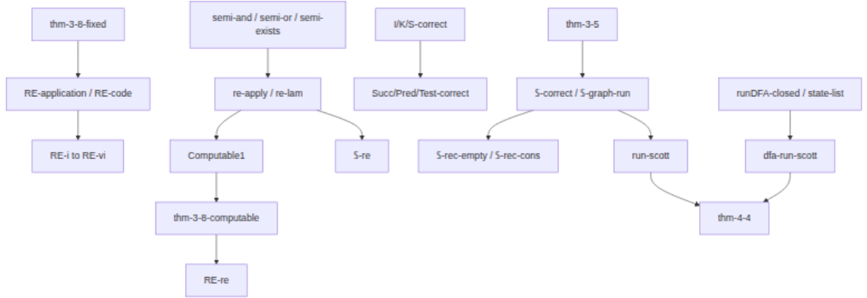
Figure 5: Recursive-enumerability, sequentializer, and Theorem 4.4 proof dependencies.
