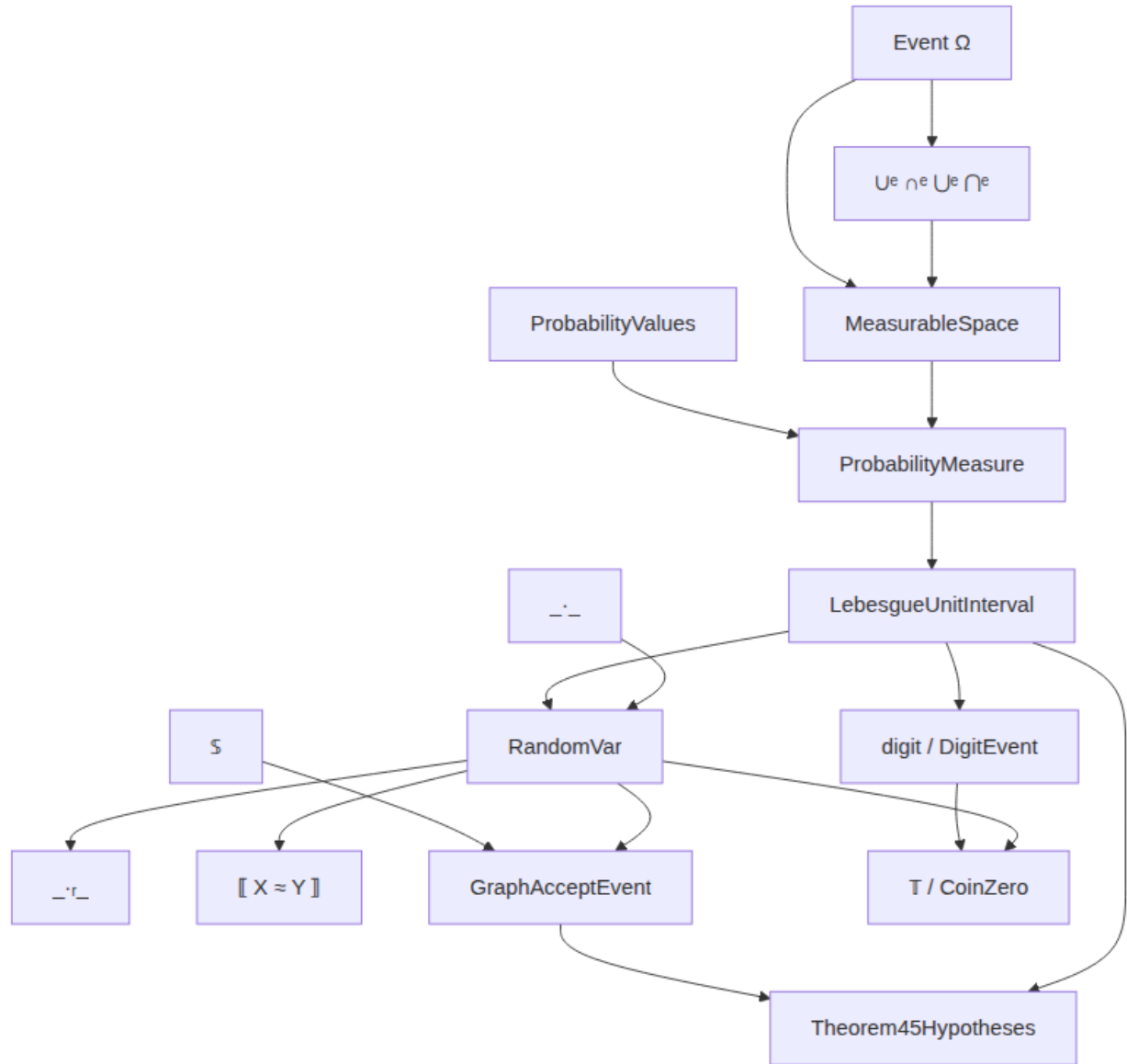
Figure 3: Relative Lebesgue and random-variable types.
