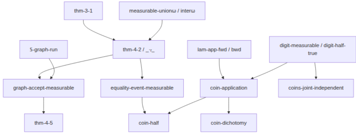
Figure 6: Literal Lebesgue proof dependencies for Theorems 4.2, 4.5, and §5.
