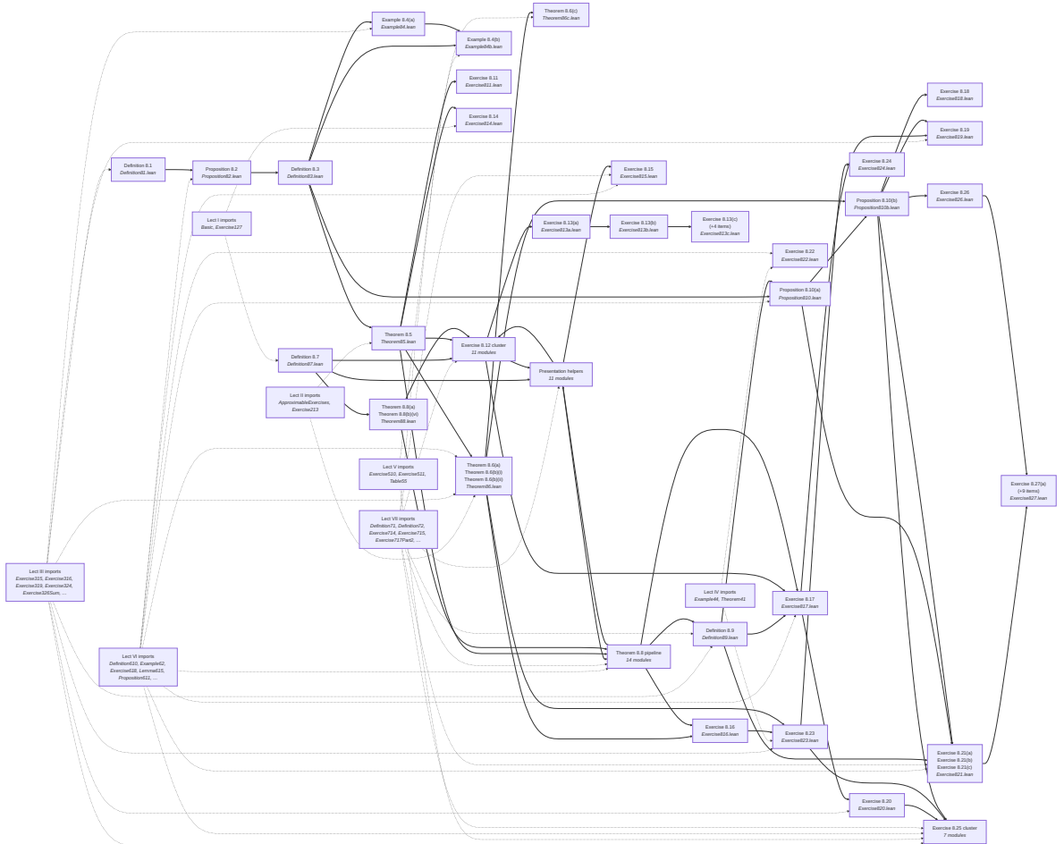
Figure 9: Lean module dependencies for Lecture VIII: Retracts of the Universal Domain.
