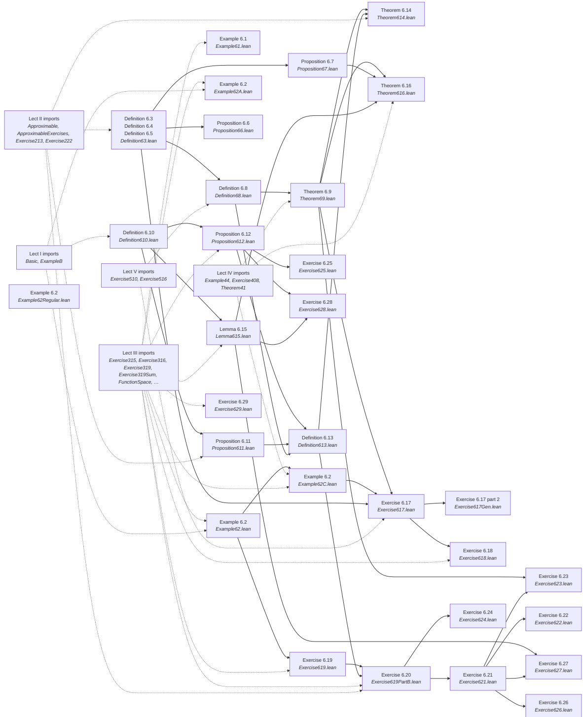
Figure 7: Lean module dependencies for Lecture VI: Domain Equations.
