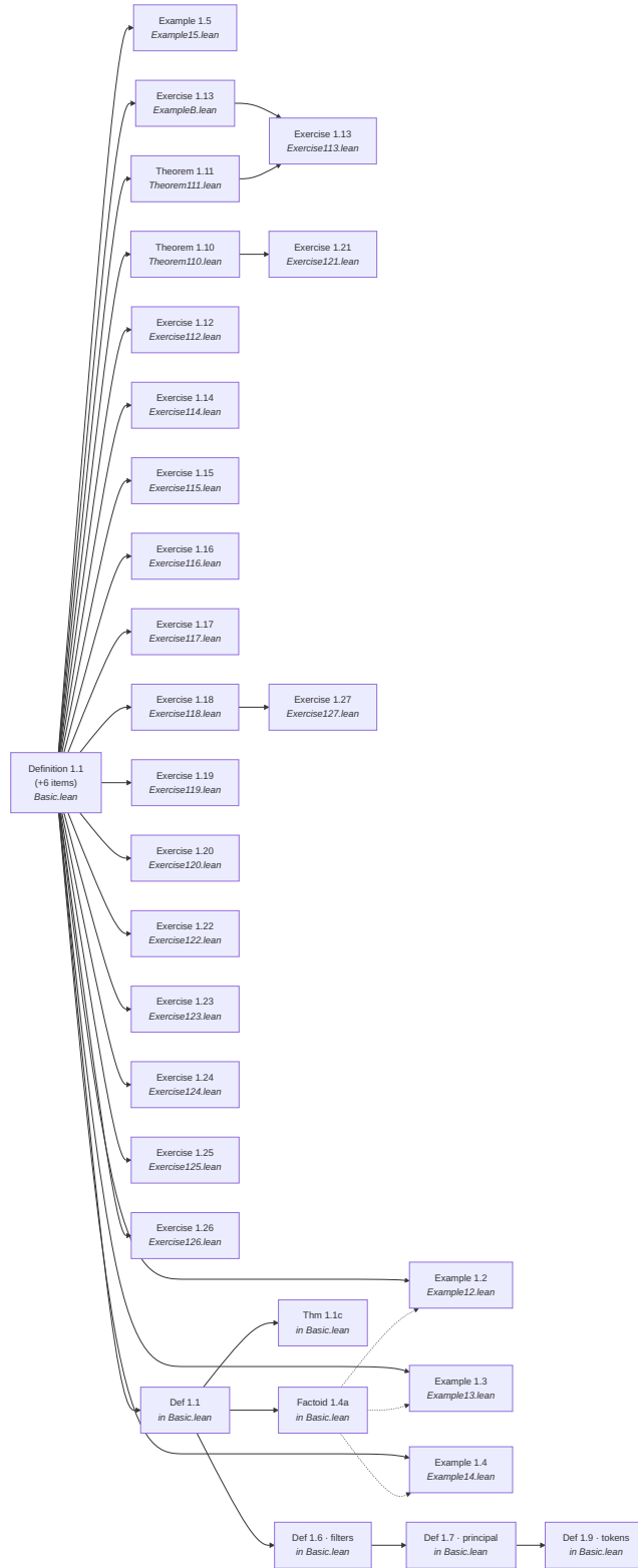
Figure 2: Lean module dependencies for Lecture I: Domains by Neighbourhoods.
