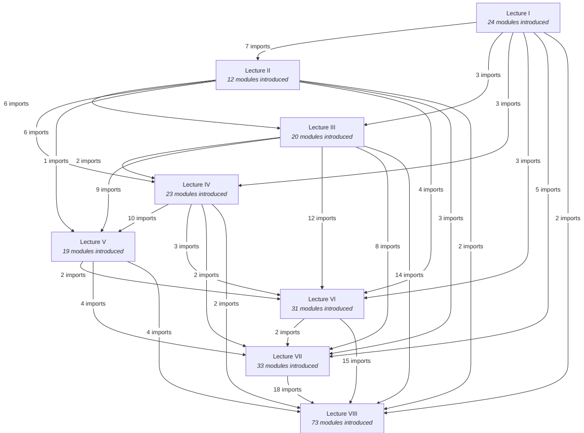
Figure 1: Chapter inclusion hierarchy (Lean imports).
