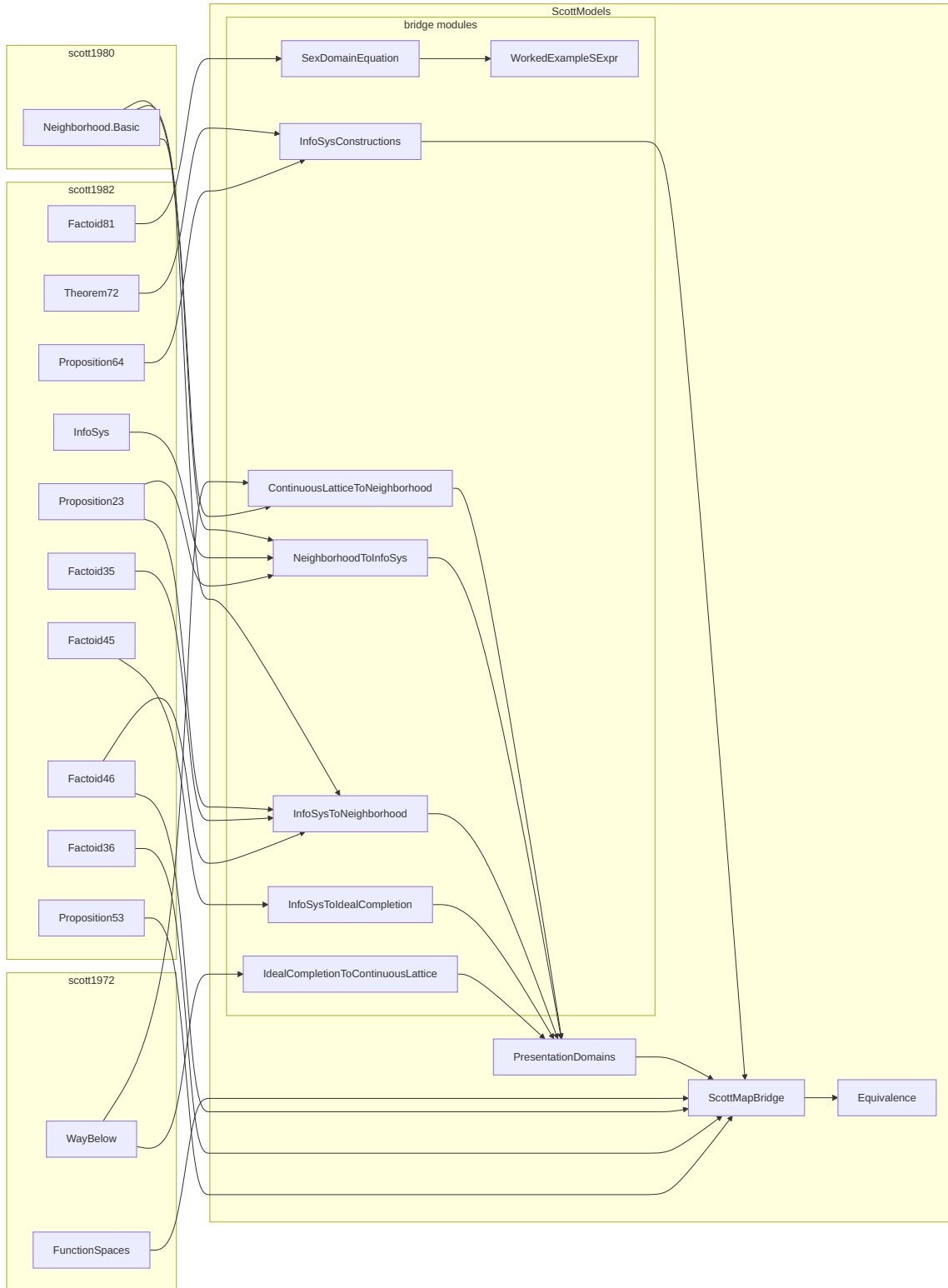
Figure 2: Catalog of bridge theorems.
