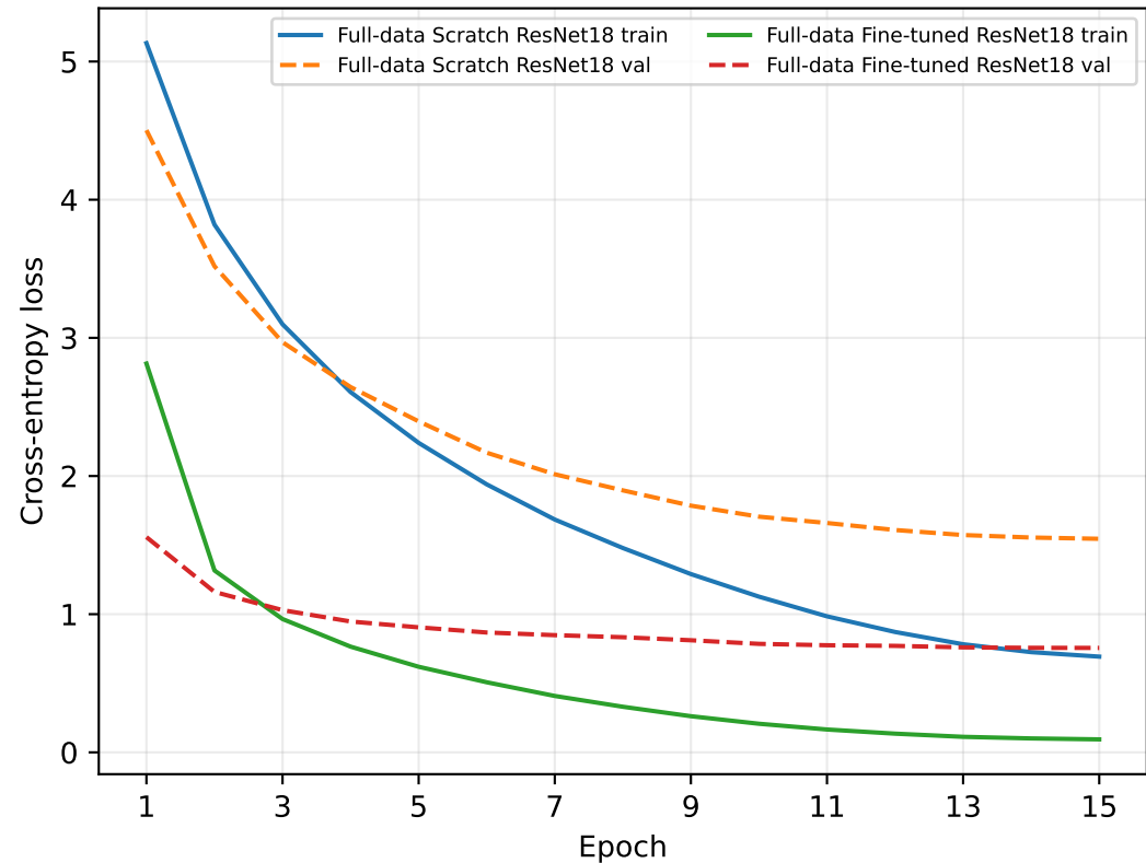
Full-data loss
