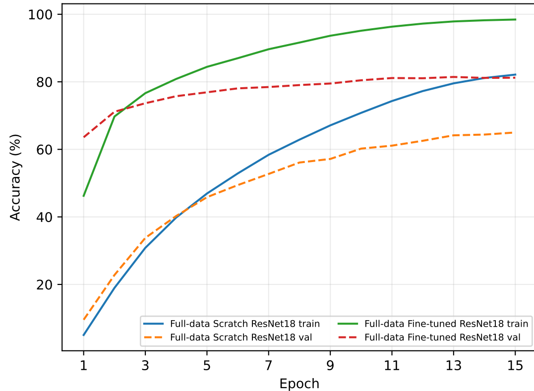
Full-data accuracy
