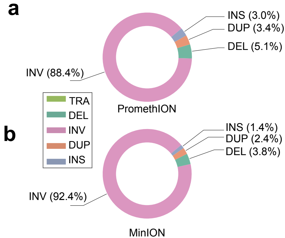
Extended Data Fig. 6 Composition of artifact-supported SVs for PromethION (a) and MinION (b). Donut charts summarize the distribution of SV types including translocation (TRA), deletion (DEL), inversion (INV), duplication (DUP), and insertion (INS) among events supported exclusively by chimera artifacts, representing artificial SVs preferentially removed by ChimeraLM(all Sniffles2 calls, without a minimum read-support filter).
