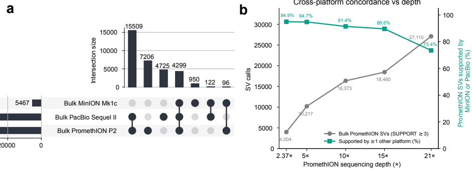
Extended Data Fig. 2 Concordance of structural variant calls among the three bulk PC3 long-read datasets. (a) UpSet plot of high-confidence SVs (Sniffles2, \geq 3 supporting reads; merged with OctopusSV) from bulk PromethION P2 (20.8x; 27,110 calls), bulk MinION Mk1c (2.4x; 5,467) and bulk PacBio Sequel II (38x; 24,655). Of the 32,907 union calls, 20,026 (60.9%) are detected on at least two platforms and 4,299 (13.1%) on all three; platform-private calls make up 26.6%, 17.4% and 19.2% of the PromethION, MinION and PacBio call sets, respectively. (b) Depth titration of the bulk PromethION data (down-sampled to 2.37x, 5x, 10x, 15x and full 21x): number of PromethION SV calls (grey) and the fraction supported by at least one of the other two platforms (teal). The platform-private fraction rises with depth (5.1% to 26.6%), showing that deeper sequencing recovers variants absent from the shallower reference sets.
