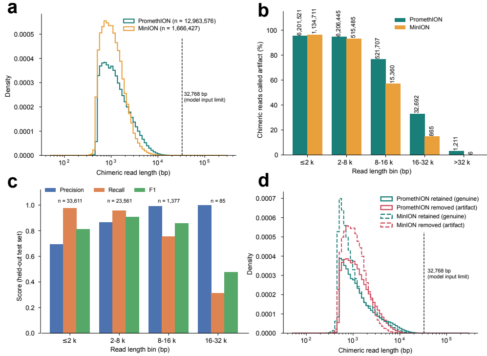
Extended Data Fig. 3 Read-length distribution of chimeric reads and length dependence of ChimeraLM classification. (a) Length distribution of chimeric reads (primary alignments carrying an SA tag) in the WGA PromethION ( n = 12,963,576 ; median 2,100 bp, N50 4,053 bp, maximum 126,974 bp) and WGA MinION ( n = 1,666,427 ; median 1,469 bp, N50 2,333 bp, maximum 42,118 bp) datasets. The dashed line marks the 32,768-bp model input limit, exceeded by 1,211 (0.009%) and 6 reads, respectively; for all but two of these reads at least one chimeric junction lies within the first 32,768 bp. (b) Fraction of chimeric reads classified as WGA-induced artifacts by read-length bin; numbers above bars give the number of reads per bin. (c) Precision, recall and F1 of ChimeraLM on WGA-derived held-out test reads ( n = 58,636 ; the 17,876 test reads sampled from bulk data are not shown because they are not part of the WGA dataset) stratified by read length. Bins with fewer than 10 reads are omitted. (d) Length distributions of chimeric reads retained (classified as genuine) and removed (classified as artifact) by ChimeraLM on both platforms (PromethION retained: median 3,087 bp, N50 7,989 bp; removed: median 2,067 bp, N50 3,836 bp; MinION retained: median 2,031 bp, N50 5,560 bp; removed: median 1,458 bp, N50 2,220 bp).
