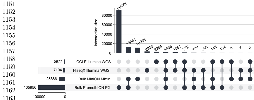
Extended Data Fig. 4 Overlap of structural variant calls among the four bulk PC3 datasets used to build the gold standard. UpSet plot of caller-consensus SVs ( \geq 2 callers per dataset) from bulk ONT MinION Mk1c (25,866 calls), bulk ONT PromethION P2 (105,956), CCLE Illumina WGS (5,977) and PRJNA361315 (HiSeq X) Illumina WGS (7,104), merged with OctopusSV. The union contains 123,115 events; 17,153 are supported by \geq 2 datasets (the gold standard used in Fig. 3), 3,029 by \geq 3 and 1,606 by all four. Within the \geq 2 set, 12,661 events (73.8%) are shared only by the two long-read datasets, 3,441 (20.1%) have both long- and short-read support and 1,051 (6.1%) are shared only by the two short-read datasets.
