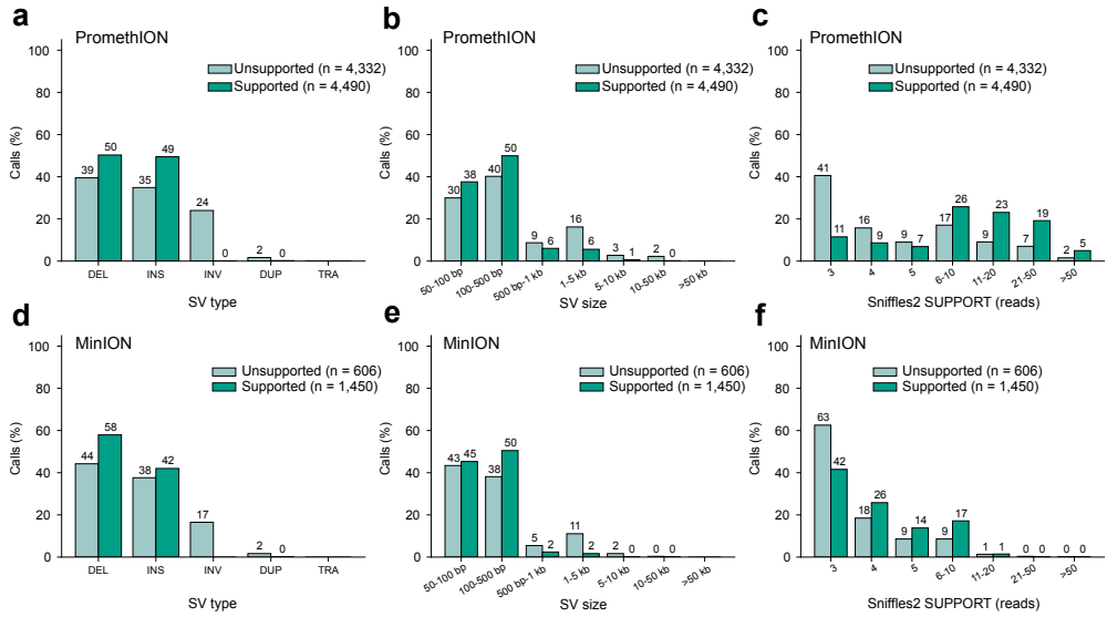
Extended Data Fig. 5 Features of structural variant calls that remain unsupported after ChimeraLM filtering. SV calls from the WGA + ChimeraLM call sets (Sniffles2, \geq 3 supporting reads) benchmarked against the gold standard (Fig. 3b,c) were split into unsupported (light teal; Truvari false positives) and supported (dark teal; Truvari true positives) calls. (a–c) PromethION ( n = 4,332 unsupported, 4,490 supported): distribution of SV type (a), SV size (b) and Sniffles2 read support (c). (d–f) The same for MinION ( n = 606 unsupported, 1,450 supported). Numbers above bars give the percentage of calls in each class.
