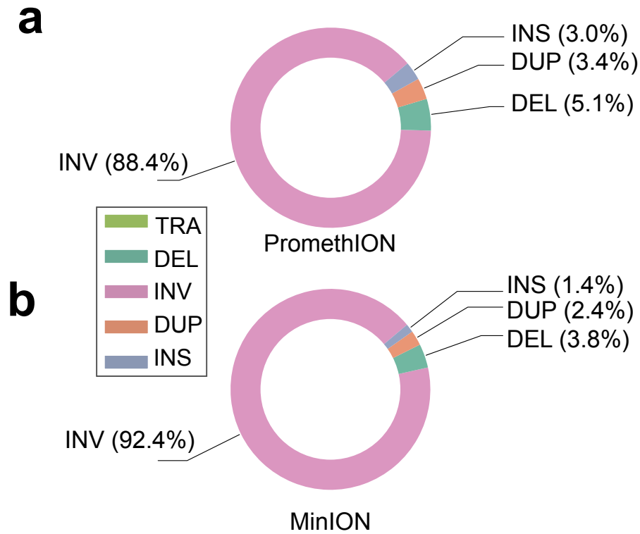
Extended Data Fig. 6 Composition of artifact-supported SVs for PromethION (a) and MinION (b). Donut charts summarize the distribution of SV types including translocation (TRA) , deletion (DEL) , inversion (INV) , duplication (DUP) , and insertion (INS) among events supported exclusively by chimera artifacts, representing artificial SVs preferentially removed by ChimeraLM.
