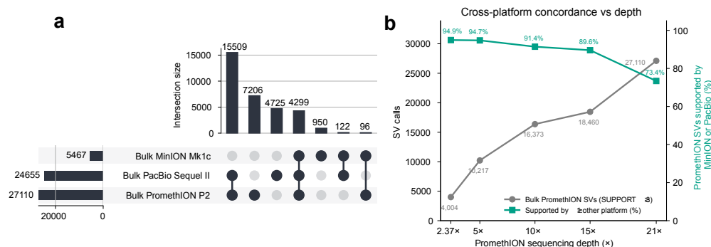
Extended Data Fig. 3 Concordance of structural variant calls among the three bulk PC3 long-read datasets. (a) UpSet plot of high-confidence SVs (Sniffles2, \geq 3 supporting reads; merged with OctopusSV) from bulk PromethION P2 (20.8x; 27,110 calls), bulk MinION Mk1c (2.4x; 5,467) and bulk PacBio Sequel II (38x; 24,655). Of the 32,907 union calls, 20,026 (60.9%) are detected on at least two platforms and 4,299 (13.1%) on all three; platform-private calls make up 26.6%, 17.4% and 19.2% of the PromethION, MinION and PacBio call sets, respectively. (b) Depth titration of the bulk PromethION data (down-sampled to 2.37x, 5x, 10x, 15x and full 21x): number of PromethION SV calls (grey) and the fraction supported by at least one of the other two platforms (teal). The platform-private fraction rises with depth (5.1% to 26.6%), showing that deeper sequencing recovers variants absent from the shallower reference sets.
