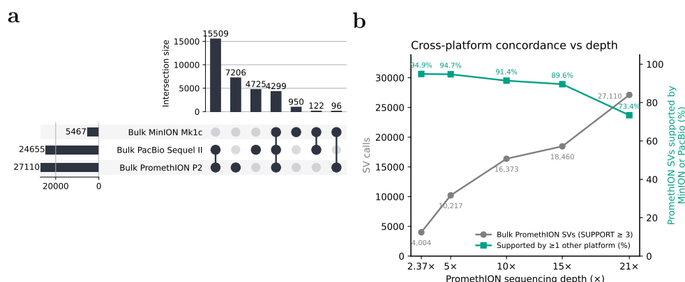
Extended Data Fig. 3 Concordance of structural variant calls among the three bulk PC3 long-read datasets. (a) UpSet plot of high-confidence SVs (Sniffles2, \geq 3 supporting reads; merged with OctopusSV) from bulk PromethION P2 (20.8 \times ; 27,110 calls), bulk MinION Mk1c (2.4 \times ; 5,467) and bulk PacBio Sequel II (38 \times ; 24,655). Of the 32,907 union calls, 20,026 (60.9%) are detected on at least two platforms and 4,299 (13.1%) on all three; platform-private calls make up 26.6%, 17.4% and 19.2% of the PromethION, MinION and PacBio call sets, respectively. (b) Depth titration of the bulk PromethION data (down-sampled to 2.37 \times , 5 \times , 10 \times , 15 \times and full 21 \times ): number of PromethION SV calls (grey) and the fraction supported by at least one of the other two platforms (teal). The platform-private fraction rises with depth (5.1% to 26.6%), showing that deeper sequencing recovers variants absent from the shallower reference sets.
