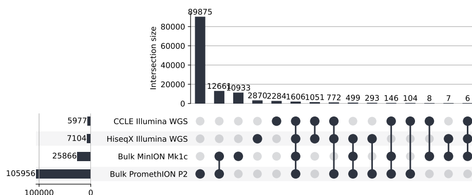
Extended Data Fig. 4 Overlap of structural variant calls among the four bulk PC3 datasets used to build the gold standard. UpSet plot of caller-consensus SVs ( \geq 2 callers per dataset) from bulk ONT MinION Mk1c (25,866 calls), bulk ONT PromethION P2 (105,956), CCLE Illumina WGS (5,977) and PRJNA361315 (HiSeq X) Illumina WGS (7,104), merged with OctopusSV. The union contains 123,115 events; 17,153 are supported by \geq 2 datasets (the gold standard used in Fig. 3), 3,029 by \geq 3 and 1,606 by all four. Within the \geq 2 set, 12,661 events (73.8%) are shared only by the two long-read datasets, 3,441 (20.1%) have both long- and short-read support and 1,051 (6.1%) are shared only by the two short-read datasets.
