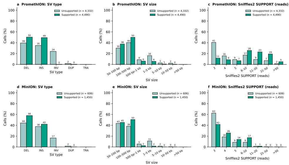
Extended Data Fig. 5 Features of structural variant calls that remain unsupported after ChimeraLM filtering. SV calls from the WGA + ChimeraLM call sets (Sniffles2, \geq 3 supporting reads) benchmarked against the gold standard (Fig. 3b,c) were split into unsupported (light teal; Truvari false positives) and supported (dark teal; Truvari true positives) calls. (a–c) PromethION ( n = 4,332 unsupported, 4,490 supported): distribution of SV type (a), SV size (b) and Sniffles2 read support (c). (d–f) The same for MinION ( n = 606 unsupported, 1,450 supported). Numbers above bars give the percentage of calls in each class.
