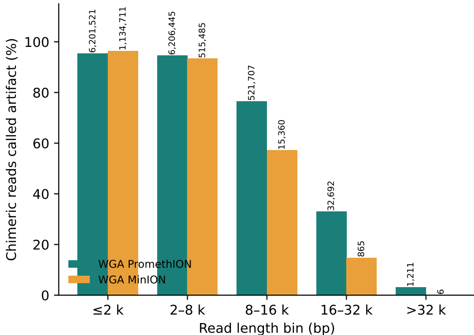
Artifact call rate by read length
