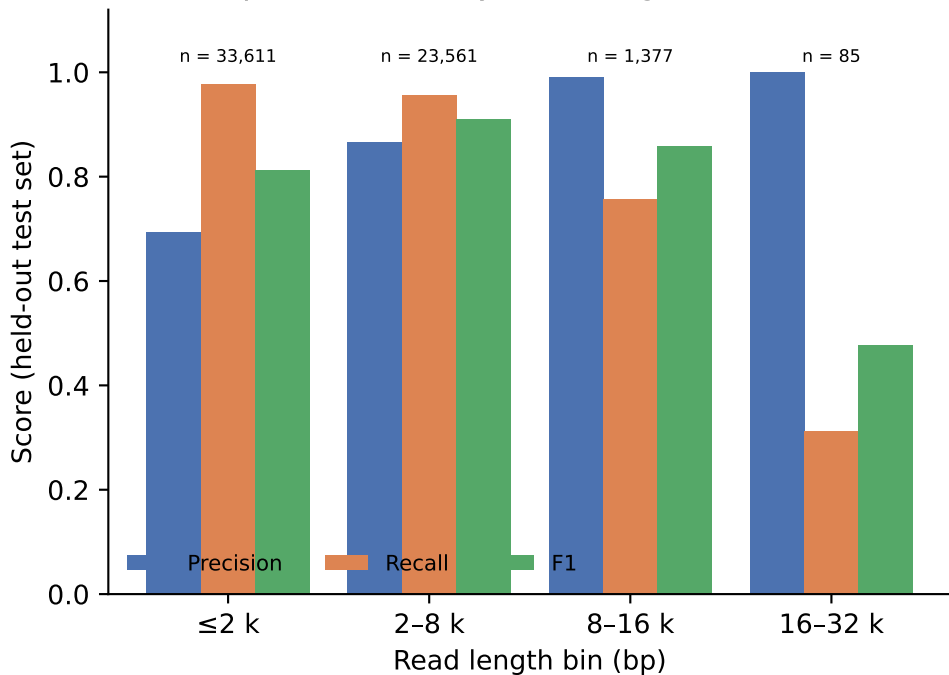
Test-set performance by read length
