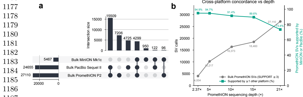
Extended Data Fig. 6 Concordance of structural variant calls among the three bulk PC3 long-read datasets. (a) UpSet plot of high-confidence SVs ( \geq 3 supporting reads; merged with OctopusSV) from bulk PromethION P2 (20.8x; 27,110 calls), bulk MinION Mk1c (2.4x; 5,467) and bulk PacBio Sequel II (38x; 24,655). Of the 32,907 union calls, 20,026 (60.9%) are detected on at least two platforms and 4,299 (13.1%) on all three; platform-private calls make up 26.6%, 17.4% and 19.2% of the PromethION, MinION and PacBio call sets, respectively. (b) Depth titration of the bulk PromethION data (down-sampled to 2.37x, 5x, 10x, 15x and full 21x): number of PromethION SV calls (grey) and the fraction supported by at least one of the other two platforms (teal). The platform-private fraction rises with depth (5.1% to 26.6%), showing that deeper sequencing recovers variants absent from the shallower reference sets.
