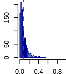
X20 (prev=7.7%)
