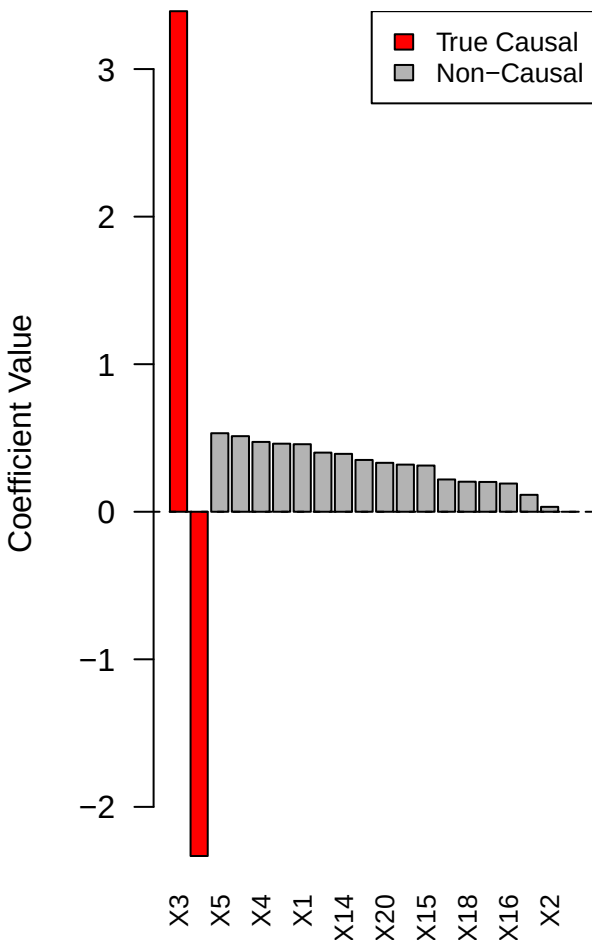
LASSO Coefficients (lambda.min)
