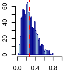
X13 (prev=13.1%)
