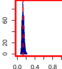
X12 (prev=13.0%)
