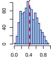
X6 (prev=29.4%)
