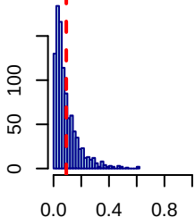
X18 (prev=9.2%)
