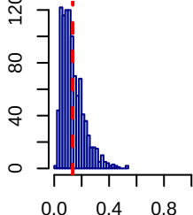
X11 (prev=13.5%)
