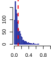
X17 (prev=10.6%)
