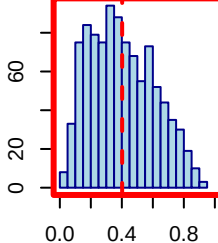
X8 (prev=27.8%)
