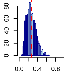
X15 (prev=16.1%)
