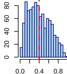
X10 (prev=26.5%)
