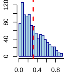
X14 (prev=19.2%)
