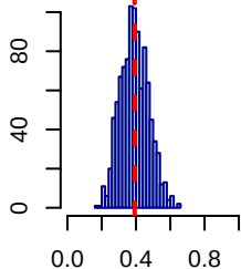
X7 (prev=25.6%)
