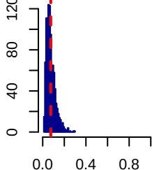
X16 (prev=7.5%)
