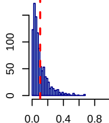
X19 (prev=10.3%)
