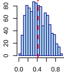
X9 (prev=31.1%)
