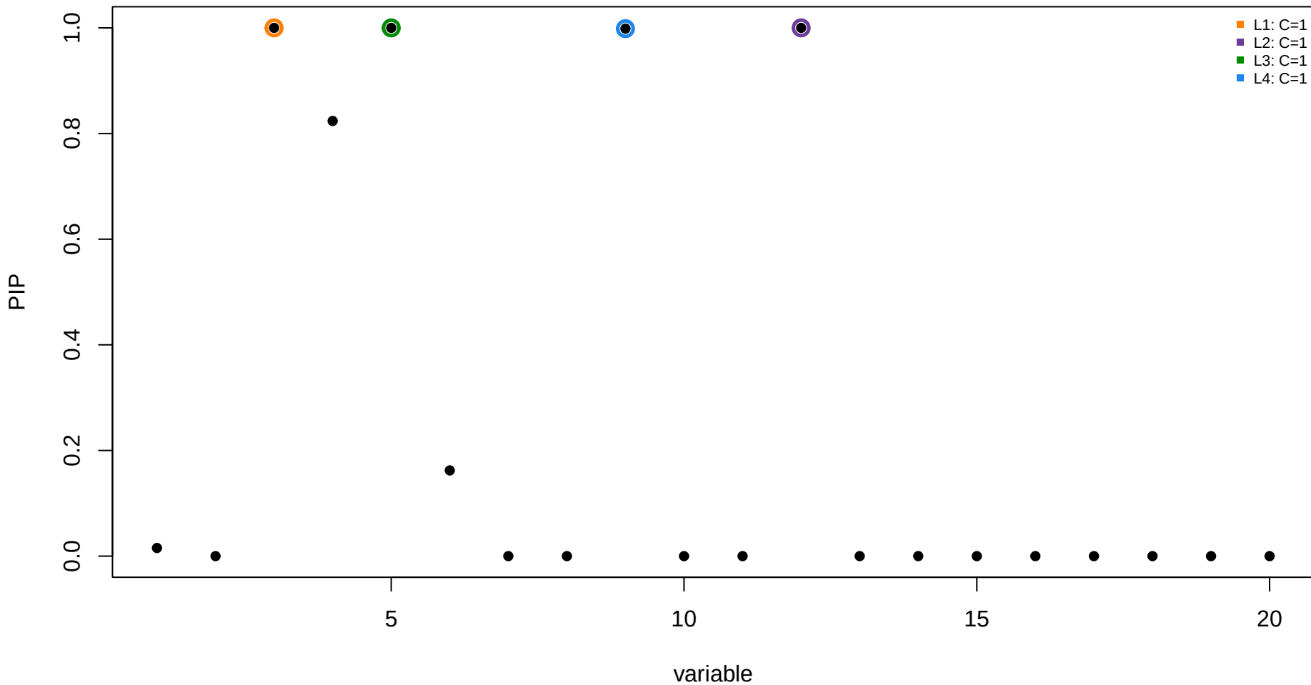
SuSiE Results (Standard Method)
