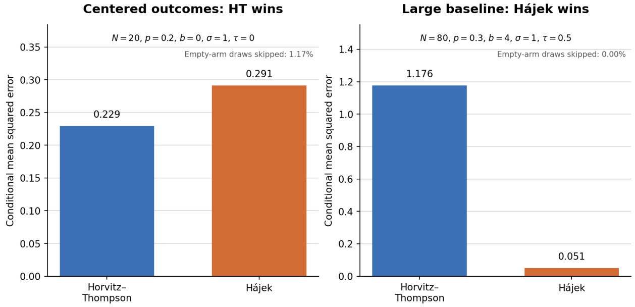
Figure 1: Two fixed simulation settings show that neither estimator uniformly minimizes finite-sample MSE. HT wins in the centered setting; Hájek wins when outcomes have a large common baseline.
