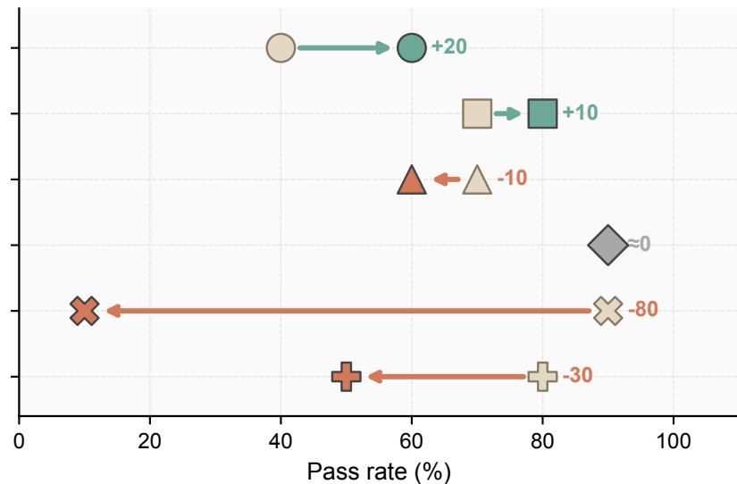
(b) L4 Direction (RID OFF → ON)
