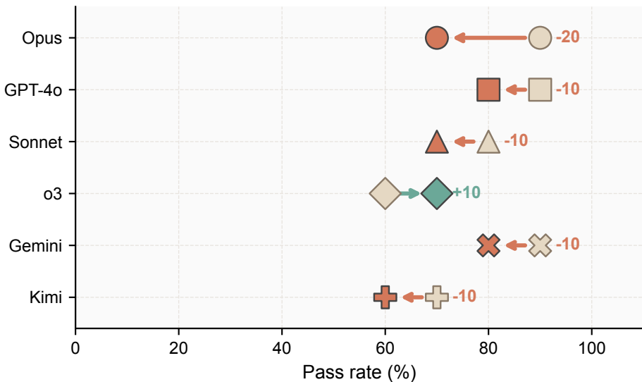
(a) L3 Strategy (RID OFF → ON)
