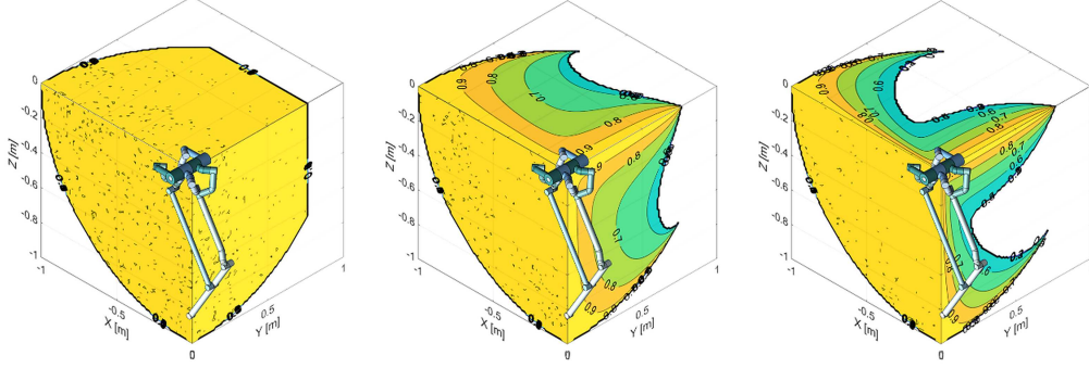
Figure 9: The contour plots shows LDI_y of the SFM when (d) |\theta_y| = 0^\circ (e) |\theta_y| = 24^\circ (f) |\theta_y| = 45^\circ
