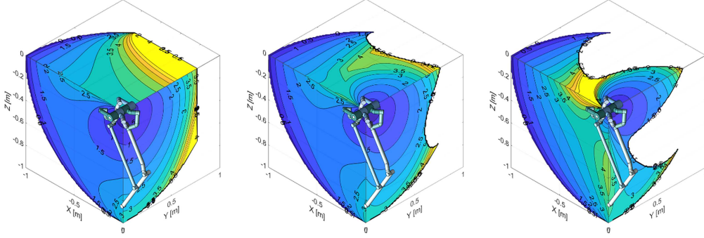
Figure 7: The contour plots shows TAR_x of the SFM when (d) |\theta_y| = 0^\circ (e) |\theta_y| = 24^\circ (f) |\theta_y| = 45^\circ
