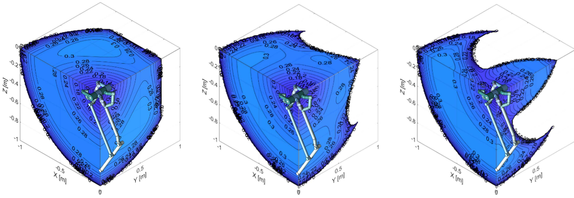
Figure 5: The contour plots shows \text{LCI}_R of the SFM when (d) |\theta_y| = 0^\circ (e) |\theta_y| = 24^\circ (f) |\theta_y| = 45^\circ
