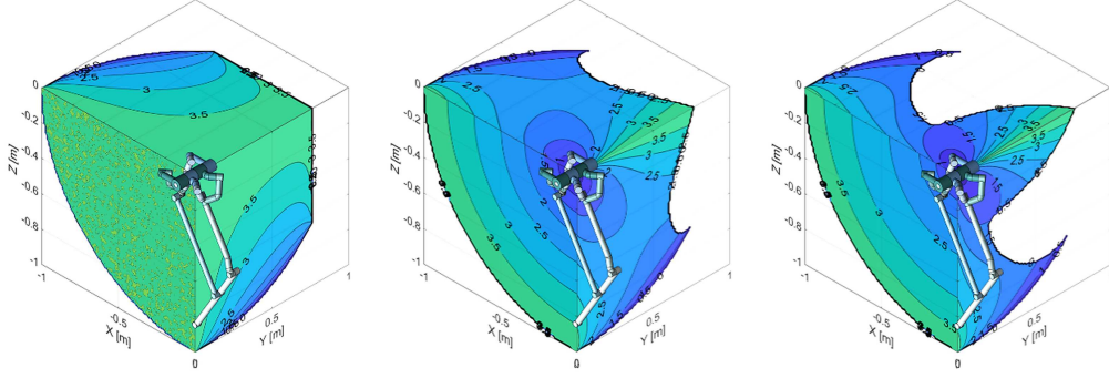
Figure 6: The contour plots shows TAR_y of the SFM when (d) |\theta_y| = 0^\circ (e) |\theta_y| = 24^\circ (f) |\theta_y| = 45^\circ
