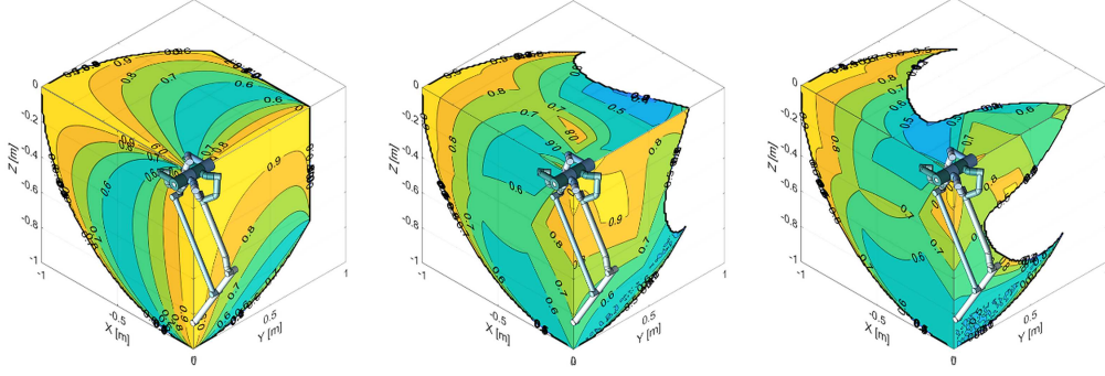
Figure 8: The contour plots shows LDI_z of the SFM when (d) |\theta_y| = 0^\circ (e) |\theta_y| = 24^\circ (f) |\theta_y| = 45^\circ
