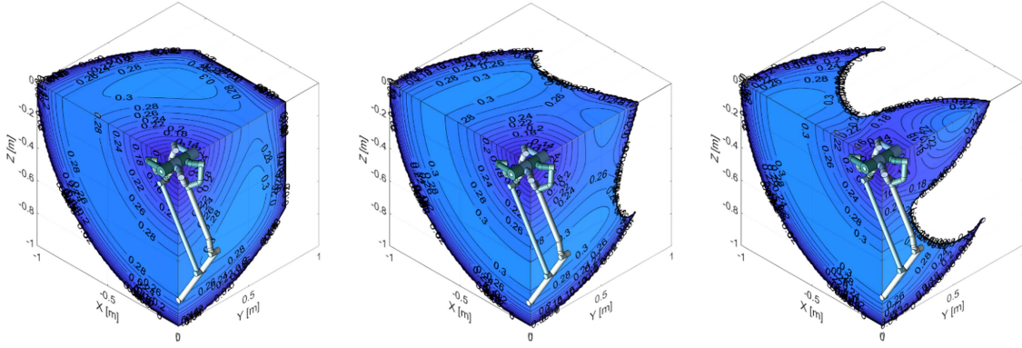
Figure 4: The contour plots shows \text{LCI}_T of the SFM when (d) |\theta_y| = 0^\circ (e) |\theta_y| = 24^\circ (f) |\theta_y| = 45^\circ
