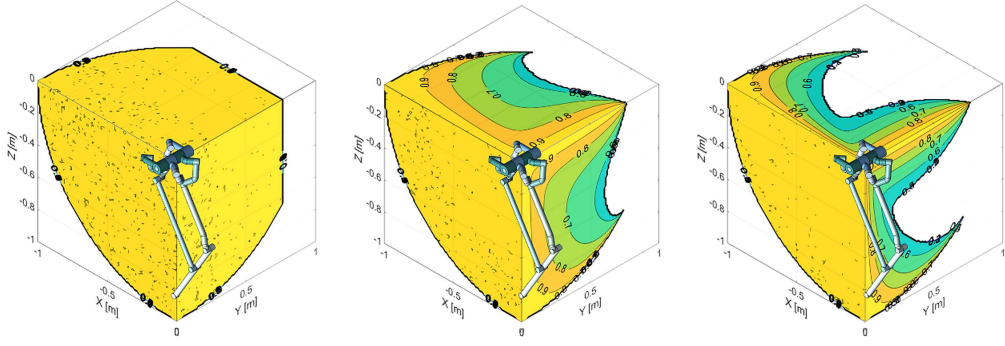
Figure 9: The contour plots shows LDI_y of the SFM when (d) |\theta_y| = 0^\circ (e) |\theta_y| = 24^\circ (f) |\theta_y| = 45^\circ
