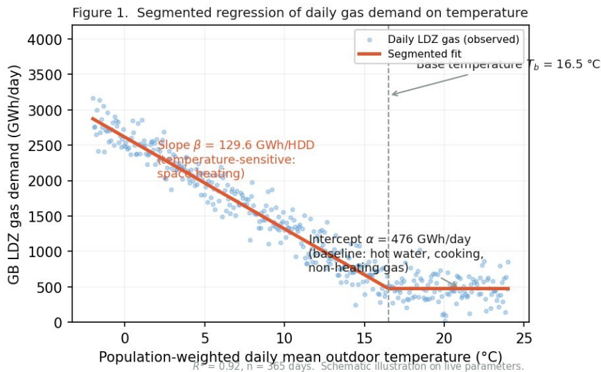
Figure 1. Segmented regression of daily gas demand on temperature. Schematic illustration on live parameters.
