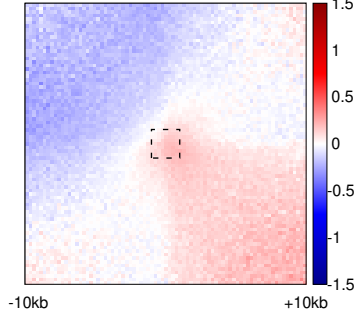
WD (n=179333)
