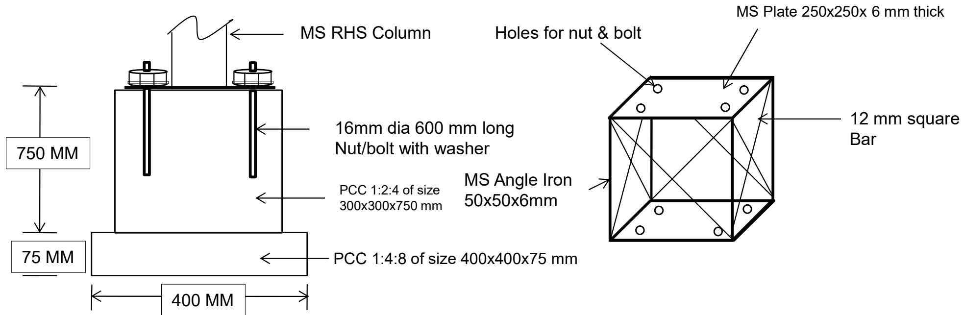
FOUNDATION DETAIL OF COLUMN
