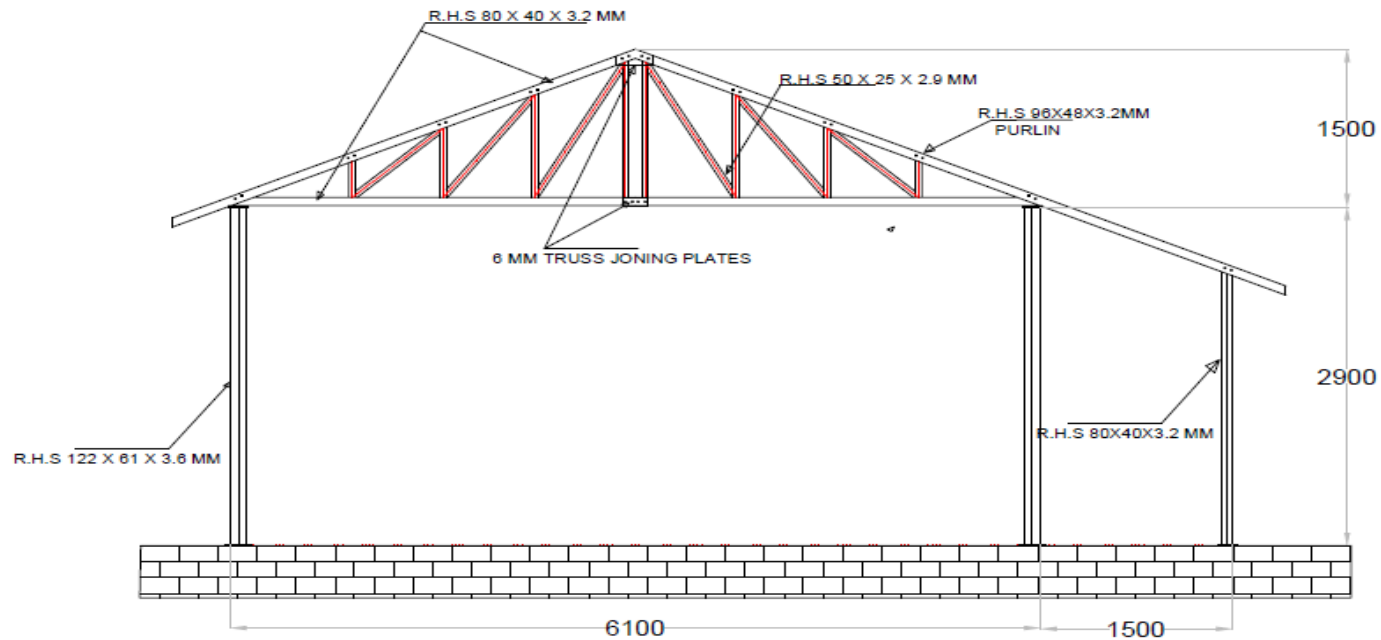
TRUSS PLAN STORE SHELTER 5.22 X 6.1 MTR
