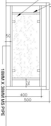
FRONT ELEVATION (FOOTBOARD)
