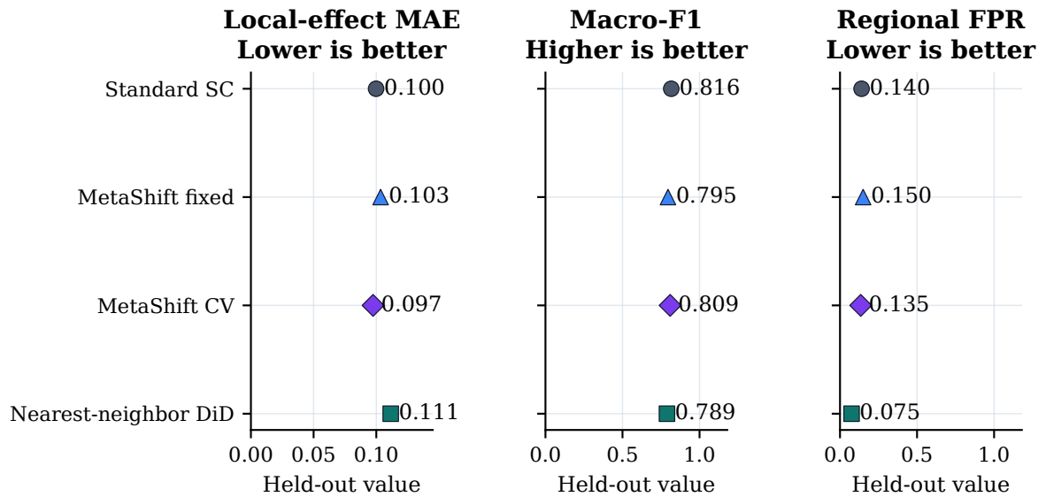
Figure 11: Held-out stable-regime synthetic comparison for the four cross-site methods. Dots show local-effect MAE, macro-F1, and regional false-positive rate on the frozen 80-site complete-input-disjoint partition; AUPRC is retained in Table 8. Lower MAE and regional false-positive rate are preferable, whereas higher macro-F1 is preferable. The panels do not form a post-hoc composite ranking; all values originate in the saved stable_full_v2 metrics table.
