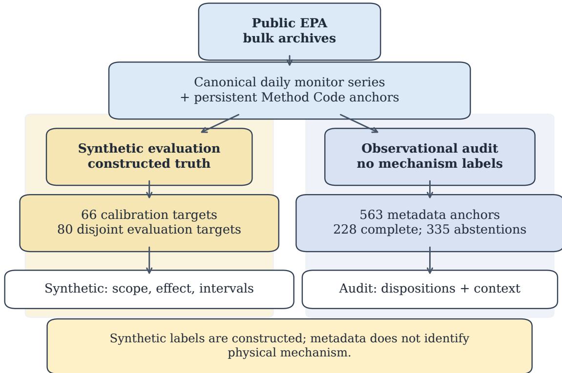
Figure 5: Frozen v0.3.2 deployment-evidence workflow. Shared preprocessing turns public archives into canonical daily series and persistent metadata anchors, then feeds separate stable-window synthetic and observational-audit lanes. The synthetic lane has labels known by construction and component-disjoint calibration/evaluation partitions; the observational lane records bounded audit dispositions and diagnostic context only. The diagram does not infer physical mechanism from metadata.
