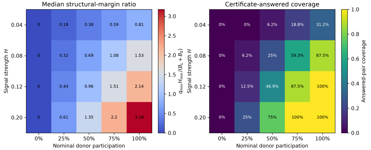
Figure 14: Supplementary normalized structural-margin phase diagram. The left panel shows median q_{\min} H_{\min}/(B_L + B_S) ; values above one meet the sufficient interval-separation condition. The right panel shows certificate answered-pair coverage. Both panels average over the five adverse comparison factors and describe the bounded synthetic construction only.
