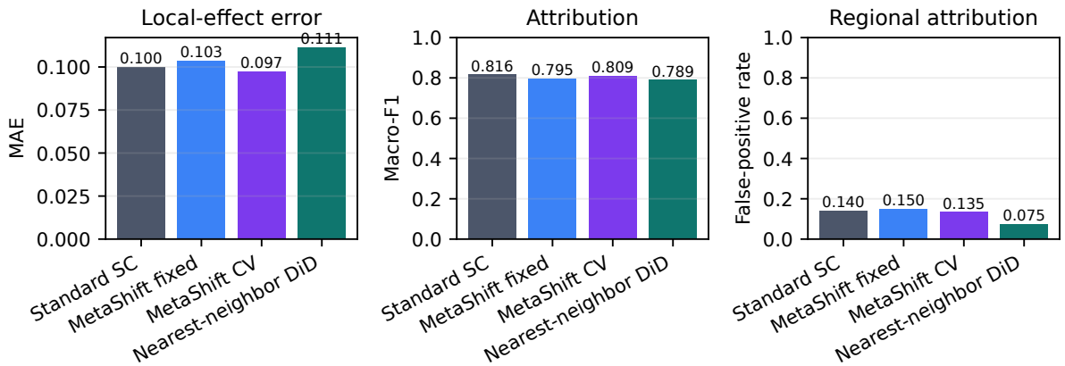
Figure 5: Held-out stable-regime synthetic metrics for the four cross-site methods. Each metric is evaluated on the frozen 80-site complete-input-disjoint partition: lower local-effect MAE and regional false-positive rate are preferable, whereas higher macro-F1 is preferable. Bars compare different criteria, not a universal ranking; all numerical values originate in the saved stable_full_v2 metrics table.
