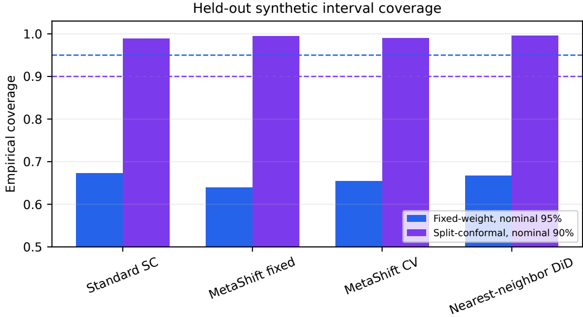
Figure 11: Empirical held-out synthetic interval coverage for four cross-site methods. Blue bars are fixed-weight conditional moving-block intervals at nominal 95%; purple bars are split-conformal intervals at nominal 90%. Dashed lines mark the corresponding nominal targets. Undercoverage and overcoverage are reported as negative calibration findings, not tuned away.
