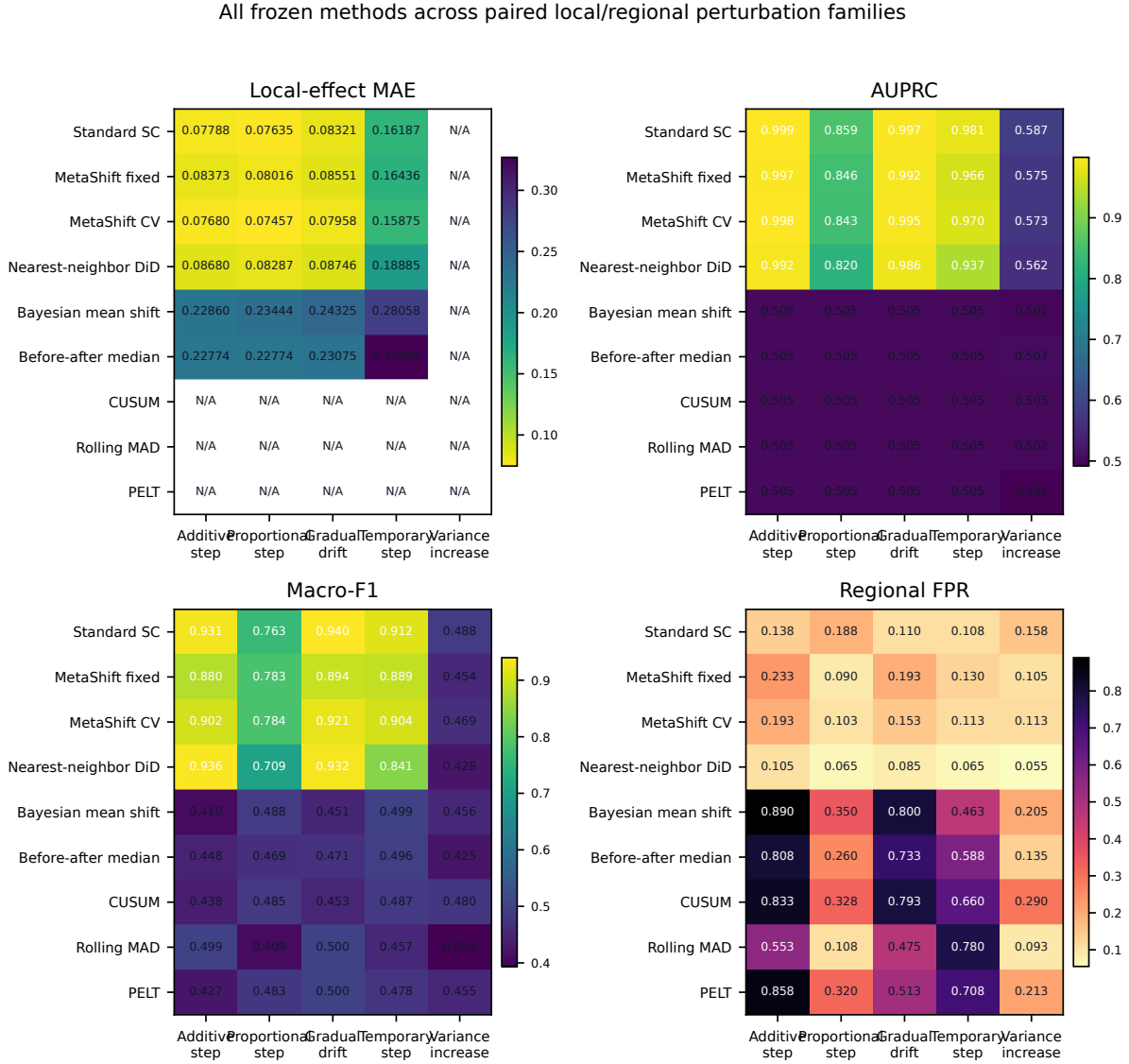
Figure 6: All nine frozen methods across the five paired local/regional perturbation families. Each cell aggregates 800 evaluation instances: a target-only local variant and a matched target-and-donor regional variant. Values are local-effect MAE, AUPRC, macro-F1, and regional false-positive rate, as labeled. N/A means that a method or variance-only condition has no defined local-effect magnitude estimate; it does not denote exclusion.
