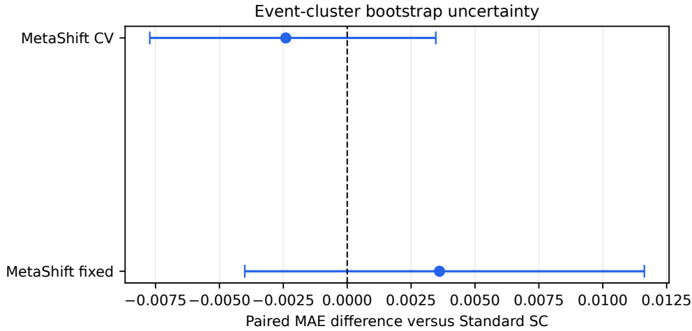
Figure 7: Paired event-cluster bootstrap intervals for MetaShift minus standard synthetic-control local-effect MAE on matched held-out synthetic instances. The dashed vertical line is no difference; negative values favor MetaShift on MAE. Both frozen intervals cross zero, so the figure does not support a confidence-supported aggregate superiority claim.
